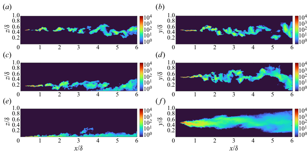
Figure 3. Instantaneous contour plot of scalar concentration \bar{c}^* from 6.25 mm source in the (x, z) plane ( a, c, e ) and (x, y) plane ( b, d, f ) for ( a, b ) the elevated source at z_s/\delta = 0.5 , ( c, d ) the elevated source at z_s/\delta = 0.19 and ( e, f ) the near-ground-level source.
