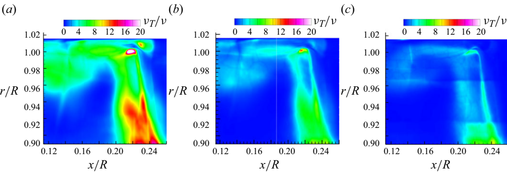
Figure 11. A contour slice in the x-r plane at the propeller trailing-edge tip R\theta/c = 0 showing the LES eddy-viscosity \nu_T normalised by the molecular viscosity \nu for (a) Grid 1, (b) Grid 2 and (c) Grid 3.
