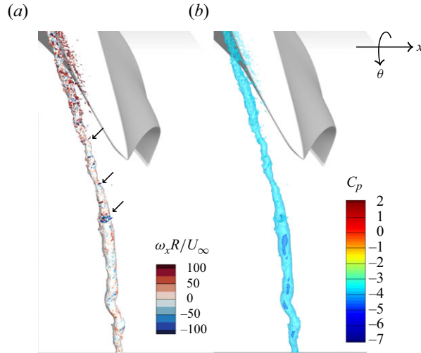
Figure 12. (a) Instantaneous isosurface of C_p = -3.7 coloured by axial vorticity \omega_x R/U_\infty . (b) Instantaneous isosurfaces of C_p = -5.5 and -3.7 are displayed transparently and coloured by C_p .
