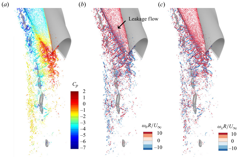
Figure 13. Instantaneous isosurfaces of Q R^2 / U_\infty^2 = 180000 coloured in (a) by the pressure coefficient C_p , (b) by the azimuthal vorticity \omega_\theta R / U_\infty and (c) by axial vorticity \omega_x R / U_\infty . An isosurface of C_p = -4.7 is also displayed in transparent grey to denote the location of the primary leakage vortex.
