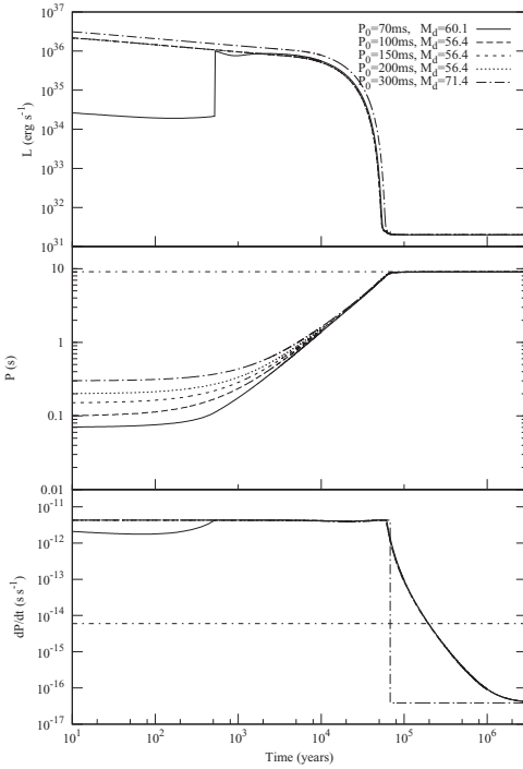
Figure 1. L_x , P and \dot{P} evolution of SGR 0418+5729: Figure 2 from Alpar, Ertan & Çalışkan (2011)
