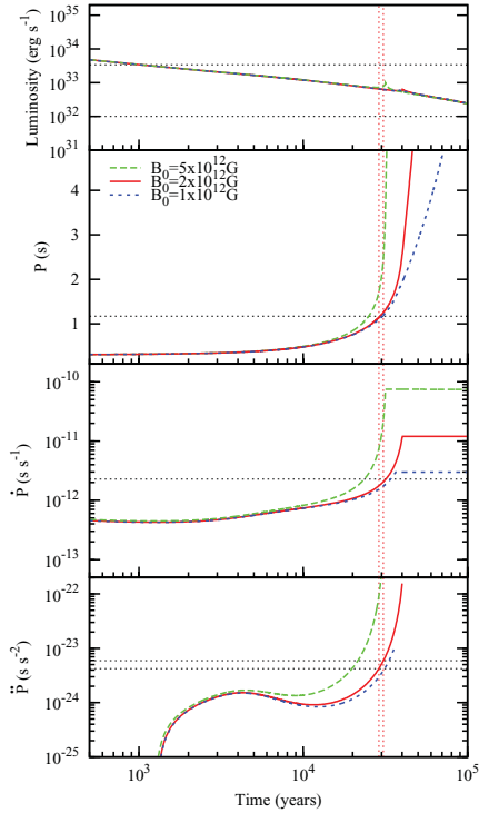
Figure 2. L_x , P , \dot{P} and \ddot{P} evolution of PSR J1734-3333: Figure 1 from Çalışkan et al. (2012)
