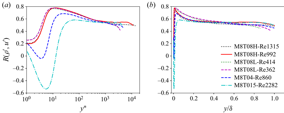
Figure 35. Correlation coefficient R(\rho', u') along the wall-normal direction plotted against (a) semi-local scaling ( y^* ) and (b) outer scaling ( y/\delta ).
