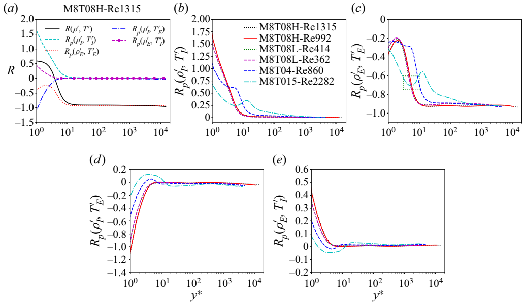
Figure 25. (a) Correlation coefficient R(\rho', T') and its relative contributions R_p(\rho'_r, T'_r) , R_p(\rho'_E, T'_E) , R_p(\rho'_I, T'_I) and R_p(\rho'_E, T'_E) along the wall-normal direction in ‘M8T08H-Re1315’. (b–e) Relative contributions (b) R_p(\rho'_r, T'_r) , (c) R_p(\rho'_E, T'_E) , (d) R_p(\rho'_I, T'_I) and (e) R_p(\rho'_E, T'_E) along the wall-normal direction in all six cases.
