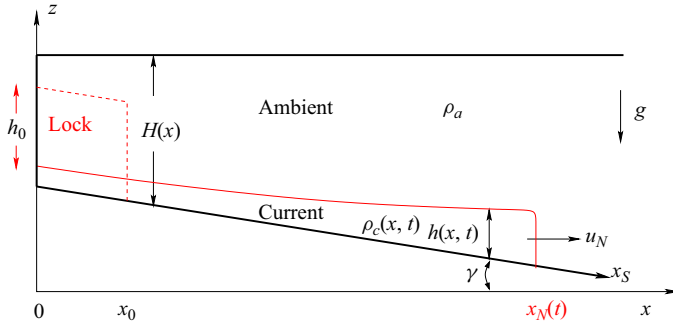
Figure 1. Sketch of the system. The GC is initially ( t = 0 ) in the lock (dashed line) of dimensions x_0, h_0 . Here x_S = x / \cos \gamma is the along-slope coordinate. (The top is usually a free surface; in the present analysis this detail is unimportant.)
