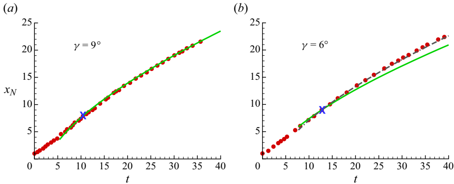
Figure 3. The x_N vs t experiment (symbols) and prediction (line) for (a) \gamma = 9^\circ and (b) \gamma = 6^\circ . The matching point is marked by X . Here c_D/E = 7 for green lines, c_D/E = 5 for the dash-dot black line in (b).
