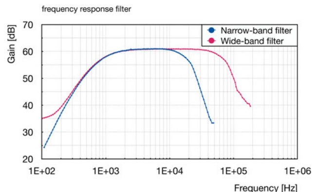
Fig. 6. Frequency response of the acoustic side receiver front end electronics.
