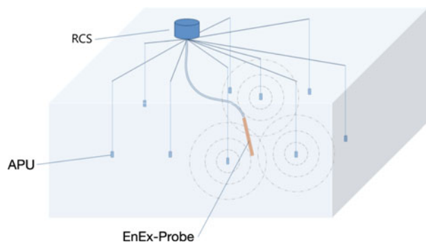
Fig. 1. Schematic mission scenario; the lander deploys the IceMole that navigates through the ice using a network of APUs.
