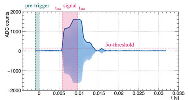
Fig. 11. Waveform of the processed acoustic signal at the distance d = 19.41 m with the signal frequency f_{\text{sig}} = 10.1 kHz; the pre-trigger and the signal region are highlighted in green and red respectively.
