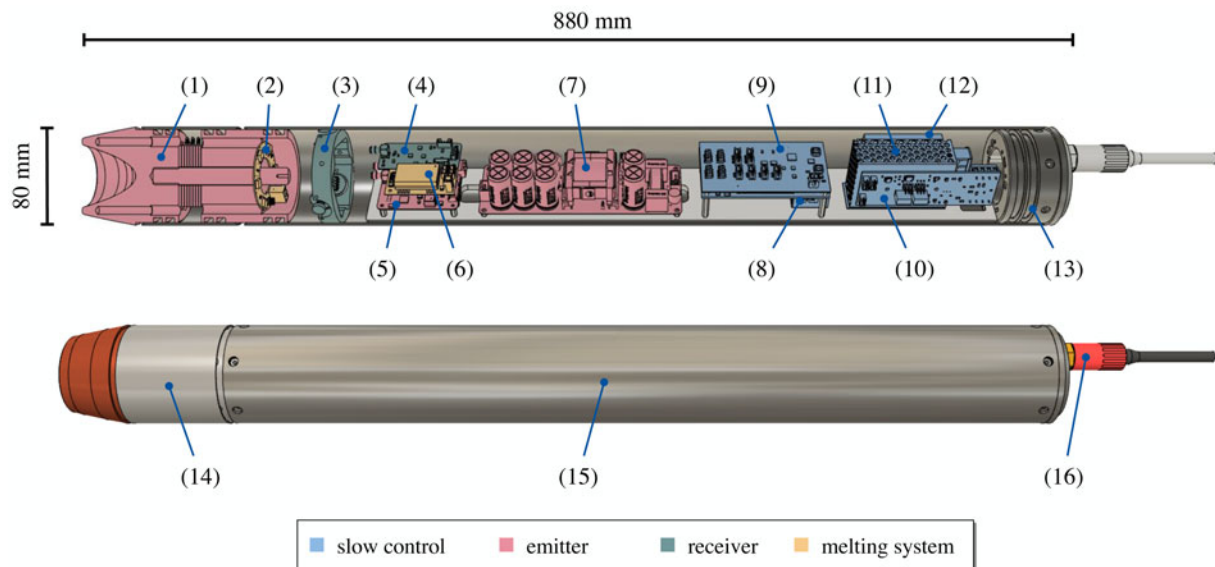
Fig. 3. Components of an APU: (1) melting head with acoustic emitter (pinger), (2) heater TRIAC ring, (3) side receivers with front end electronics, (4) front receiver front end electronics, (5) pinger front end electronics, (6) heater controller, (7) pinger power supply, (8) MicroZed SoC module, (9) SoC carrier board, (10) power monitor and synchronization module, (11) low voltage power supply, (12) power line communication adapter, (13) sealing end with back heater, (14) pinger hull, (15) main hull and (16) external connector (cabling omitted for clarity).
