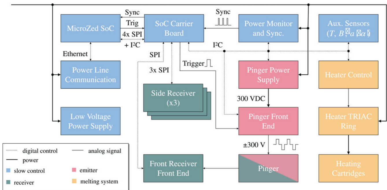
Fig. 4. Block diagram of an APU containing slow control, emitter, receiver and melting system; low voltage power supply connections (12, 5 and 3.3 V) are omitted for clarity.
