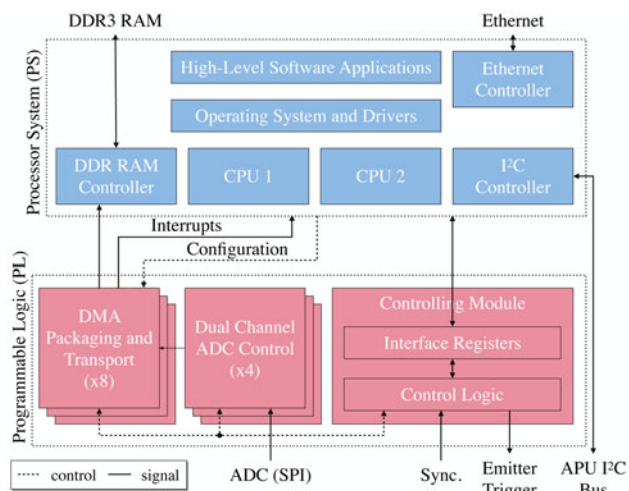
Fig. 9. Structure of the implemented firmware modules in the programmable logic.
