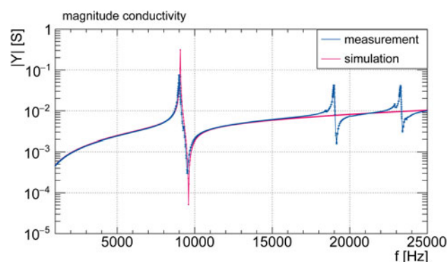
Fig. 8. Simulation and measurement of the electrical conductivity showing the (anti-) resonances of the pinger; also the absolute off-resonance conductivity is correctly predicted over the full range. The two visible higher order resonances have not been included in the simulation.
