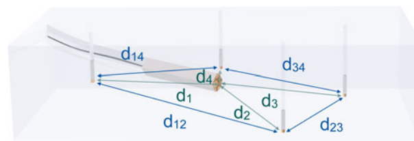
Fig. 2. Illustration of trilateration within the acoustic network consisting of four APUs and the IceMole.
