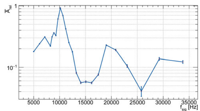
Fig. 12. Transfer characteristic of acoustic signals in the acoustic navigation network between APUs in glacial ice.
