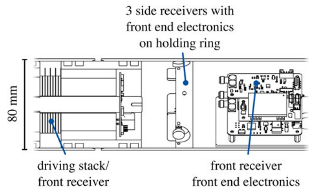
Fig. 5. Detail view of the APU front and side receivers.
