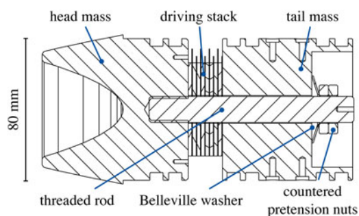
Fig. 7. APU melting head including the tonpilz transducer assembly in cross-sectional view.
