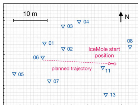
Fig. 14. 2D projection of the experimental setup for the navigation verification; shown are the APUs of the acoustic navigation network with their corresponding number (blue), the start position of the IceMole (red) and the planned trajectory (dotted line).
