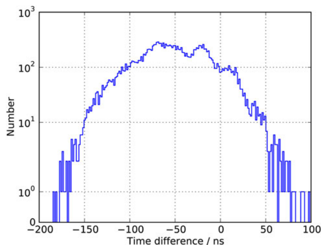
Fig. 10. Distribution of the time difference between the rising edges of the synchronization signals of two different synchronization modules used for the APUs and the APS; the standard deviation is 39 ns.
