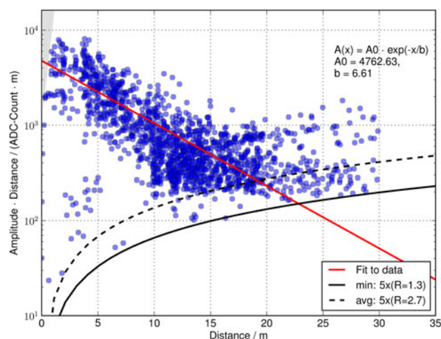
Fig. 15. Visualization of the overall performance of the APU network during the field test 2018; See text for details.
