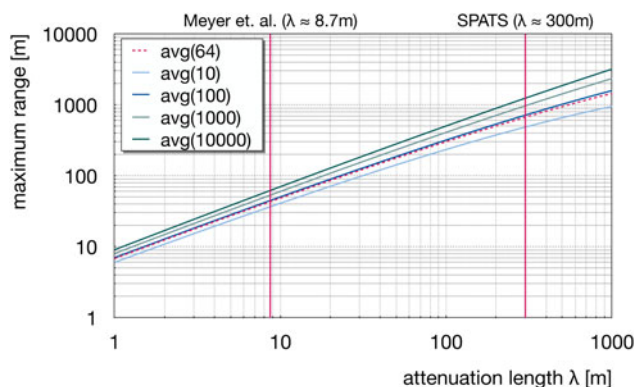
Fig. 13. Range estimation with respect to the attenuation in ice; shown are different curves for the different number of averages. The dotted red line shows the configuration used in EnEx-RANGE. The solid red lines mark the attenuation lengths measured at the Langenferner glacier (Meyer and others, 2019) and the cold ice of Antarctica (Abbasi and others, 2011).
