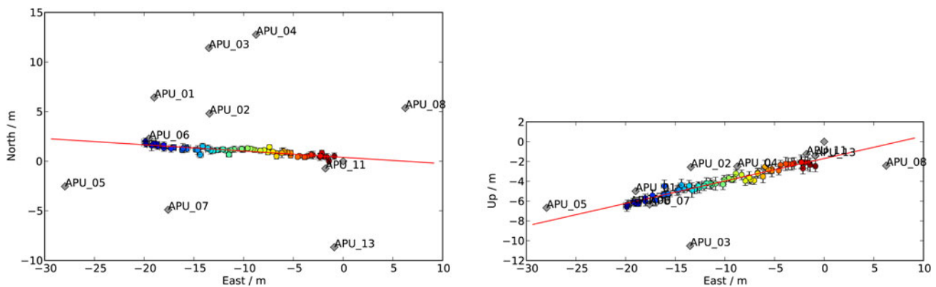
Fig. 16. Reconstruction of the positions of the IceMole during the EnEx-RANGE field test; the reconstructed positions are represented by the colored dots. The colors encode the time increasing from red to blue. The grey diamonds labeled with APU_01 to APU_13 are the positions of the emitters. The red line represents the resulting trajectory.
