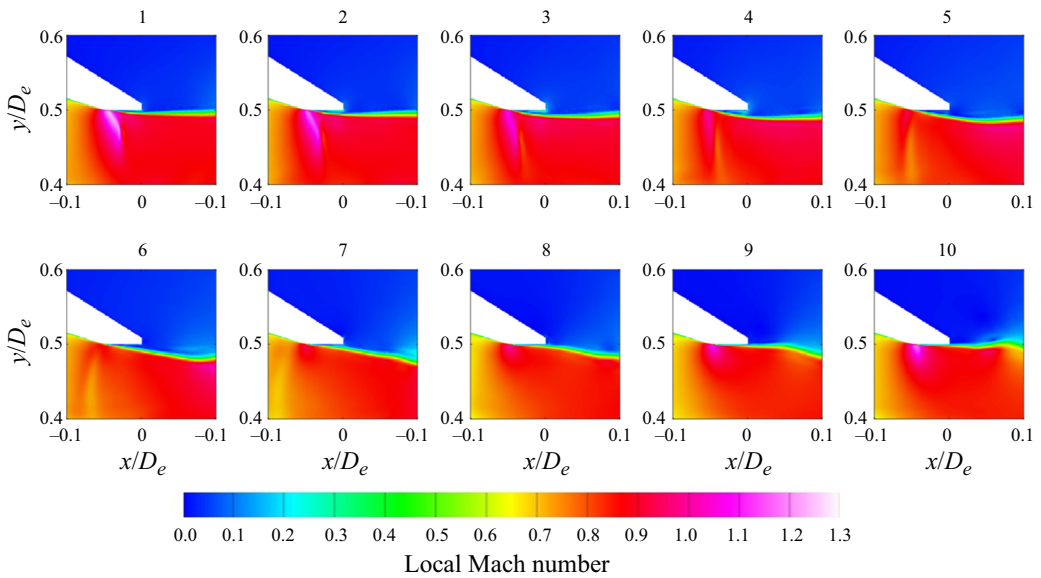
Figure 12. Snapshots from HRLES simulation showing instantaneous distributions of local Mach number. L_e/D_e = 0.7, M_j = 0.90 , unheated.
