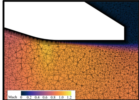
Figure 6. Cross-sectional views of the computational grid used: (a) view of computational domain with nozzle coupled to plenum chambers on left and (b,c) detailed view of the grid inside the nozzle near final-nozzle exit. Colour in (b,c) shows time-averaged local Mach number for M_j = 0.90 , unheated operating condition.
