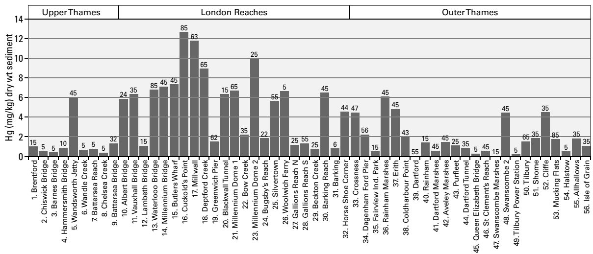
Figure 2 (A) Spatial distribution of Hg in surface sediments of the Thames estuary. (B) Spatial distribution of maximal Hg from shallow sediment cores of the Thames estuary. See Table 3 for explanation of Action Level 2. Values above columns correspond to the specific depth interval from surface (in cm).
