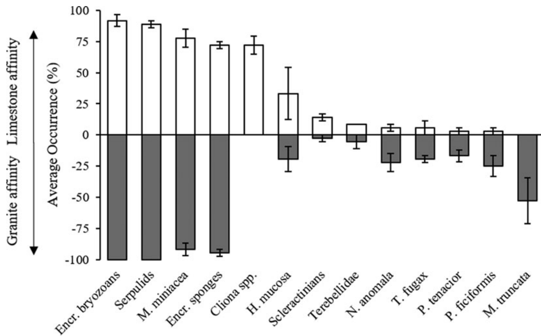
Fig. 3. Lithological affinity of species/OTUs \pm SE present in all the sites of at least one substrate. White bars, limestone; grey bars, granite.
