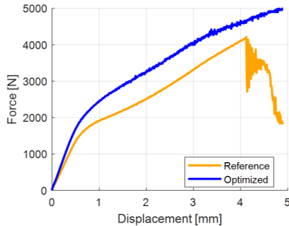
Figure 4. Virtual Test on component level
