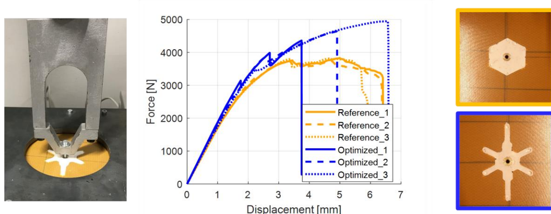
Figure 7. Physical test on substructure level
