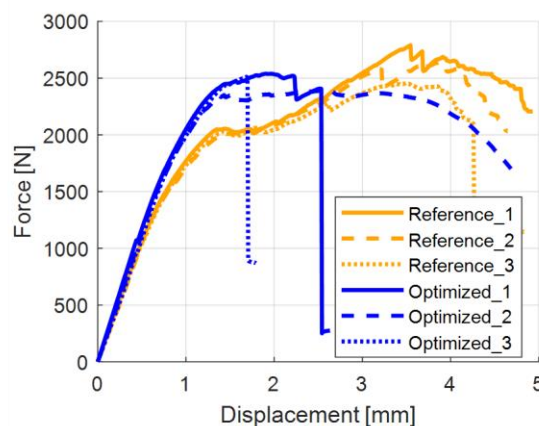
Figure 5. Physical test on component level
