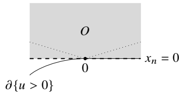
Figure 4. Asymptotic expansion in nontangential cone plus monotonicity also gives control in \{x_n \leq 0\} .
