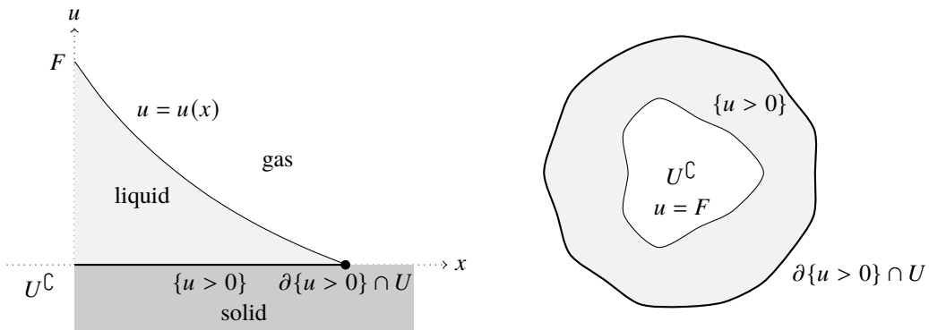
Figure 1. Side view (left) and the top view (right) of the setup for the one-phase free boundary problem.
