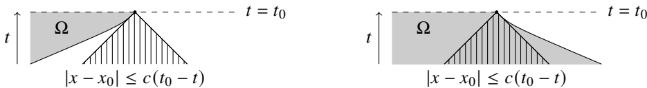
Figure 5. Left: velocity c cone touches \Omega(t) from the outside at (t_0, x_0) , interpreted as V_n(t_0, x_0) \geq c . Right: velocity c cone touches \Omega(t) from the inside at (t_0, x_0) , interpreted as V_n(t_0, x_0) \leq -c .
