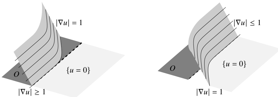
Figure 3. Left: Obstacle from above, slope is larger than 1 everywhere and saturates where free boundary bends into O . Right: Obstacle from below, slope is smaller than 1 everywhere and saturates where free boundary bends away from \overline{O}
