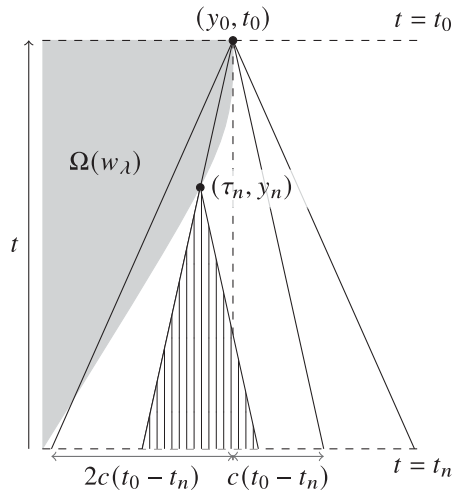
Figure 6. Space-time picture displaying the definition of (\tau_n, y_n) .
