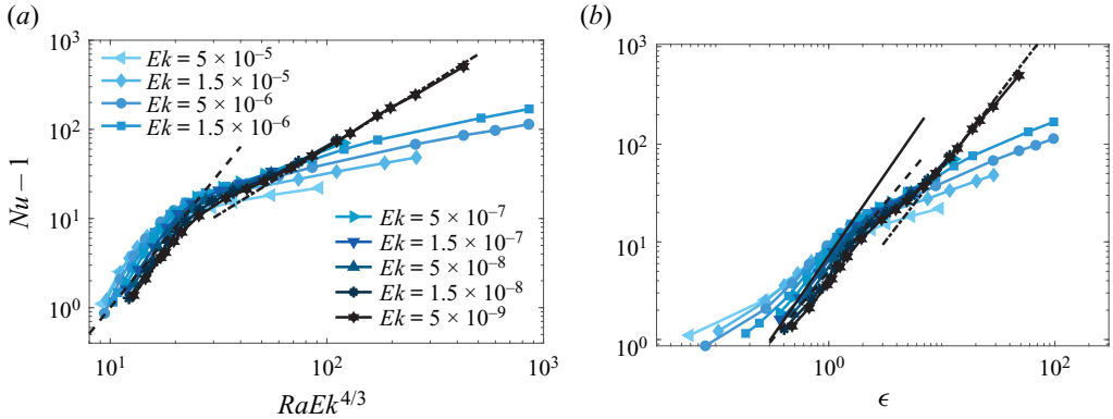
Figure 12. Convective heat transport Nu - 1 versus (a) the supercriticality RaEk^{4/3} and (b) the \epsilon = Ra/(8.7Ek^{-4/3}) - 1 for all the DNS data shown in figure 2. The dashed line in (a) denotes the steep heat transfer scaling of Nu - 1 \sim 0.001Ra^3Ek^4 and the dash-dotted line the asymptotic heat transfer scaling of Nu - 1 \sim 0.06Ra^{3/2}Ek^2 . The dashed line in (b) denotes the scaling of Nu - 1 = 5\epsilon^{1.4} , the solid line Nu - 1 = 2.2\epsilon + 3.5\epsilon^2 proposed by Ecke (2015), and the dash-dotted line the asymptotic heat transfer scaling of Nu - 1 \sim 1.8\epsilon^{1.5} .
