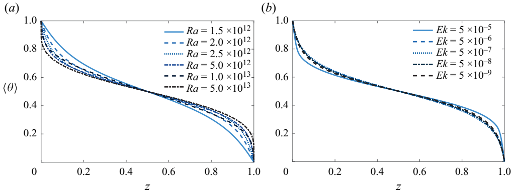
Figure 5. Vertical profiles of the time and horizontally averaged temperature \langle \theta \rangle for ( a ) different Ra and fixed Ekman number Ek = 5 \times 10^{-9} and ( b ) different Ekman numbers and similar Nusselt numbers 10.6 \leq Nu \leq 12.3 .
