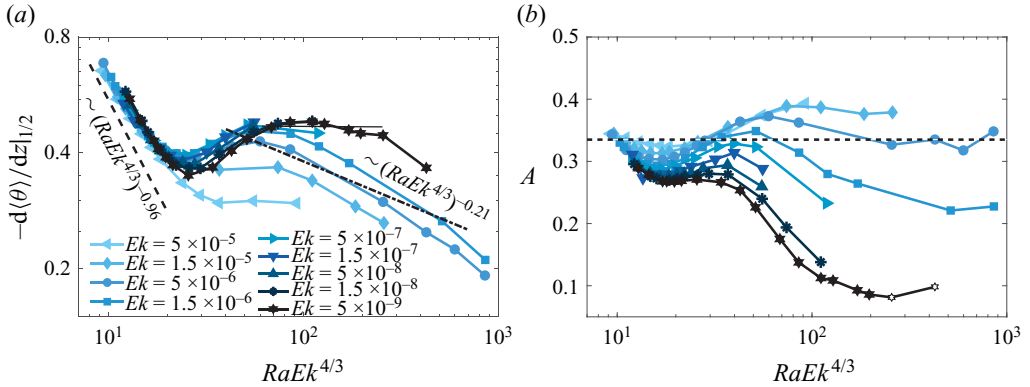
Figure 6. (a) Temperature gradient at middle height as a function of RaEk^{4/3} for different Ek . The horizontal solid line denotes a flattened range of the smallest Ek . The dashed line represents the scaling of (RaEk^{4/3})^{-0.96} proposed by Julien et al. (2012b), the dash-dotted line denotes the scaling of (RaEk^{4/3})^{-0.21} for rotation-influenced turbulence demonstrated by Cheng et al. (2020) in experiments. (b) Kinetic energy anisotropy A = u_z^2/(u_h^2 + u_z^2) as a function of RaEk^{4/3} for different Ek . The horizontal dashed line ( A = 1/3 ) denotes isotropy.
