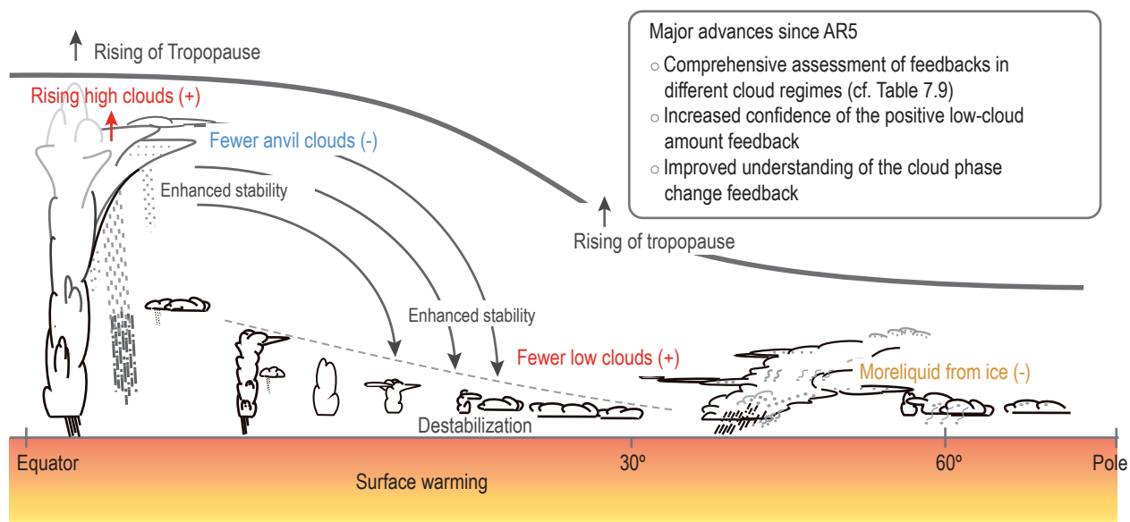
Figure 7.9 | Schematic cross section of diverse cloud responses to surface warming from the tropics to polar regions. Thick solid and dashed curves indicate the tropopause and the subtropical inversion layer in the current climate, respectively. Thin grey text and arrows represent robust responses in the thermodynamic structure to greenhouse warming, of relevance to cloud changes. Text and arrows in red, orange and green show the major cloud responses assessed with high , medium and low confidence, respectively, and the sign of their feedbacks to the surface warming is indicated in the parenthesis. Major advances since AR5 are listed in the box. Figure adapted from Boucher et al. (2013).
