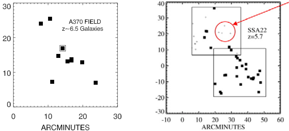
Figure 5. (Left) The z \sim 6.55 emitters in A370 display a filamentary extent. The box indicates a z \sim 6.74 galaxy, currently the highest confirmed redshift. (Right) Redshift z \sim 5.7 structure in the expanded SSA22 field. Small crosses (circled region) show candidates not yet spectroscopically observed along the extended filament.
