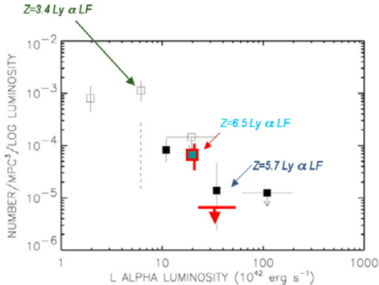
Figure 3. The Ly \alpha luminosity function of identified z \sim 5.7 galaxies ( filled boxes ) compared with the Ly \alpha luminosity functions at z \sim 3.4 ( open boxes ) (Cowie & Hu 1998; Hu et al. 1999). Measured points are shown with 1\sigma Poisson uncertainties based on the number of objects in each bin. The vertical dashed line indicates the limits of the z \sim 5.7 survey, which does not extend to the faint end of the z \sim 3.4 Ly \alpha luminosity function. The points and upper limits for the z \sim 6.5 luminosity function are shown with the thick bars, and are consistent with the z \sim 5.7 luminosity function, but are based on only 14 galaxies.
