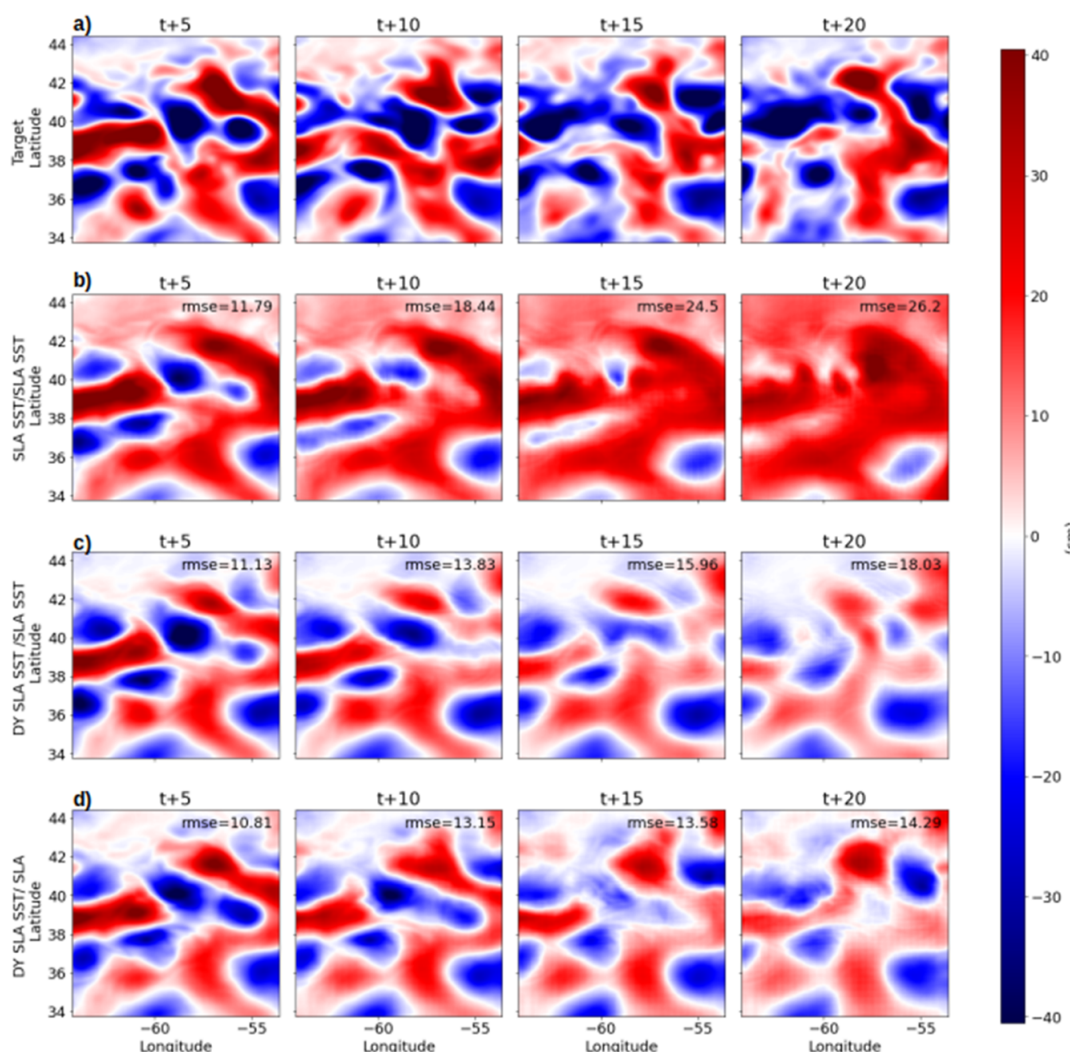
Figure 6. SLA image predictions at time t + 5 day; t + 10 days; t + 15 days; t + 20 days ( t = 24/10/1993 ). (a) correspond to the ground truth results, (b) to the SLA-SST/SLA-SST method, (c) correspond to the DY SLA-SST/SLA-SST method, and (d) to the DY-SLA-SST/SLA method.
