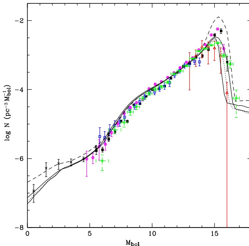
Figure 4. Luminosity functions obtained from the SDSS catalogue: Black solid squares (Harris et al. 2006), open blue squares, only DAs (DeGennaro et al. 2008), black crosses (Krziesinski et al. 2009), and green stars (Munn et al. 2017). Magenta stars were obtained from the SCSS catalogue (Rowell & Hambly (2011)) and contain DA and non-DA stars. The two solid black lines are the theoretical luminosity function, obtained assuming a constant SFR and an age of 10 and 13 Gyr, respectively, while the dashed line corresponds to a decreasing exponential SFR and the dotted line to a constant SFR with an exponential tail.
