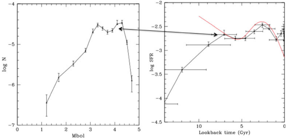
Figure 8. Left panel: empirical luminosity function of massive ( M_{WD} \leq M/M_{\odot} \leq 1.1 ) DA white dwarfs in the solar neighborhood ( Tremblay et al. 2019 ). Right panel: the corresponding star formation rate ( Isern 2019 ), in red, the Galactic disc star formation ( Mor et al. 2019 ).
