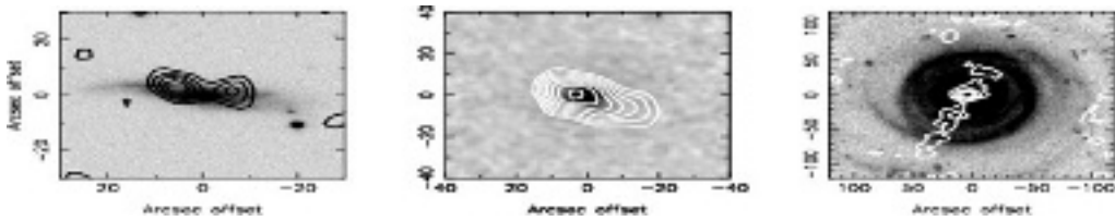
Figure 1. The panel shows 610 MHz observations of all three galaxies. From left to right (a) PGC 045080: Contours levels are 2, 3, 4, 5 times the noise level where the map noise is \sigma = 0.12 \text{ mJy beam}^{-1} and beam is 7'' ; (b) UGC 1922: Contours levels are 12, 14, 16, 18, 20, 22, and 24 \sigma where \sigma = 0.49 \text{ mJy beam}^{-1} and the beam is 24'' ; (c) UGC 6614: Contours levels are 3, 5, 7, 9 and 11 \sigma where \sigma = 0.25 \text{ mJy beam}^{-1} and the beam is 15'' .
