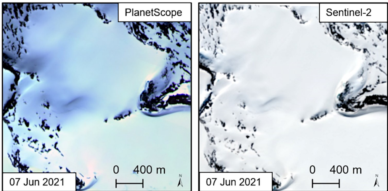
Fig. 10. Comparison of the PlanetScope and Sentinel-2 image quality during the early ablation season. The maps show that the PlanetScope image suffers from illumination disturbances due to the snow cover, while the quality of the Sentinel-2 image is more consistent.
