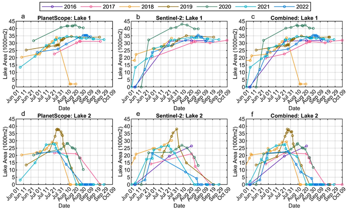
Fig. 5. Development of the areas of Lakes 1 and 2 at Tystigreen throughout the ablation seasons of 2016-22. The two plots on the left (a,d) show the results based on maps derived from the PlanetScope imagery, the two plots in the middle (b,e) show lake areas derived from the Sentinel-2 imagery, and the plots on the right (c,f) show the combined results of PlanetScope- and Sentinel-2-derived lake areas.
