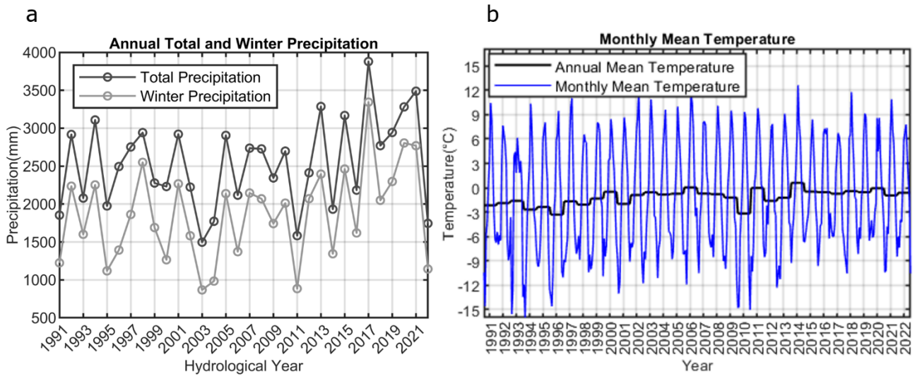
Fig. 2. Multi-decadal evolution of the annual and winter precipitation (a), and annual and monthly mean temperature (b) at Tystigbreen for the period of 1991-2022 derived from the national gridded dataset seNorge (Lussana and others, 2019). The hydrological year is defined as the period from September 1 to August 31 (NVE, 2020). Here, “winter precipitation” refers to the accumulation season between October 1 and April 30.
