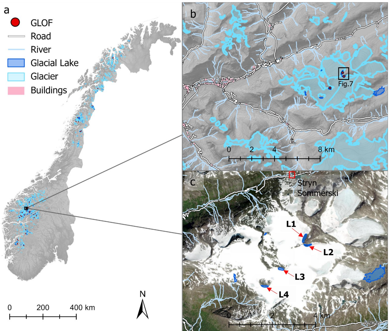
Fig. 1. Map of the study area showing (a) the distribution of glaciers and glacial lakes in Norway, (b) map of the study area of Tystigbreen and downstream areas with previously documented GLOF-generating glacial lakes, and (c) Worldview-2 satellite image of Tystigbreen (30 July 2021) with the confirmed and newly identified drainage-prone ice-dammed lakes (Lakes 1 – 4 marked as L1-L4) and the location of the Stryn Summer Ski centre testing a citizen-based data collection for this project.
