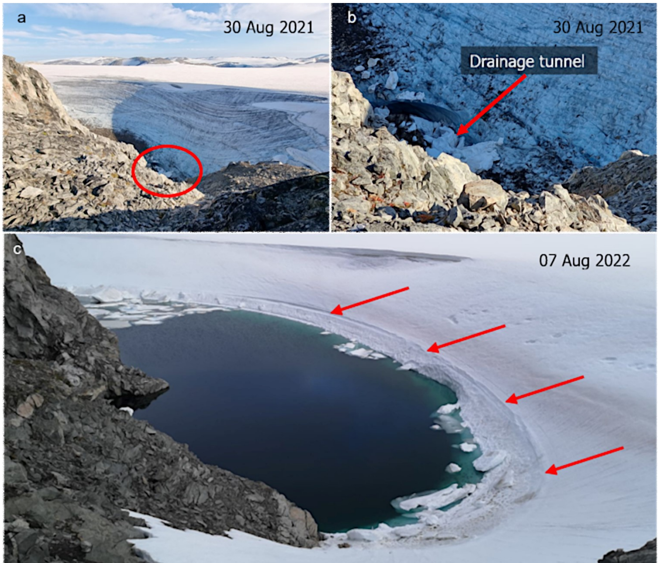
Fig. 8. Detected drainage of Lake 2 in August 2021 (a and b). The location of the drainage tunnel in (b) is indicated with a red circle (a). (c) shows the onset of drainage of Lake 2 in August 2022. The arrows indicate the maximum water level. Photos: Stryn Summer Ski.
