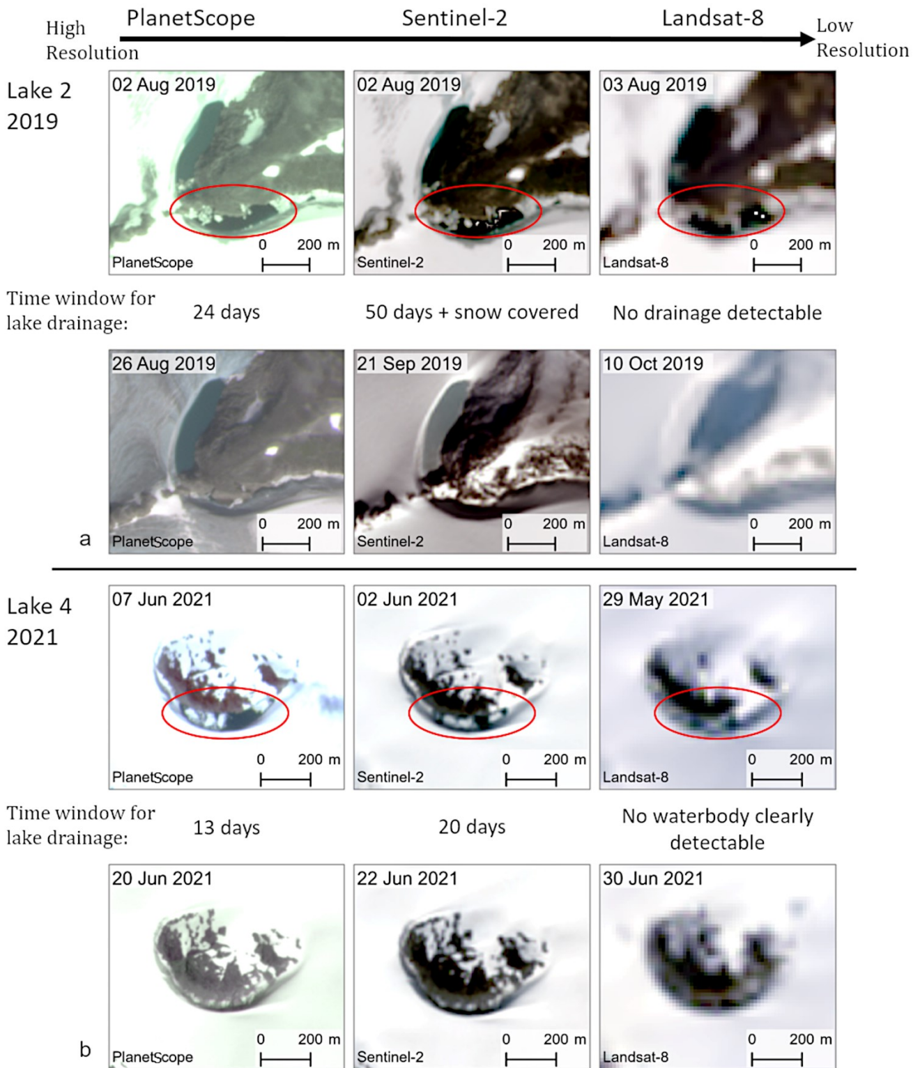
Fig. 4. Detectability of Tystigbreen's glacial lakes in the PlanetScope (left), Sentinel-2 (middle) or Landsat-8 (right) imagery, including the time window constraining the glacial lake drainages for each satellite product. The upper two panels (a) show an example of the drainage event from Lake 2 in 2019. The lower two panels (b) depict the drainage of Lake 4 in 2021. Projection: WGS1984 UTM Zone 32N.
