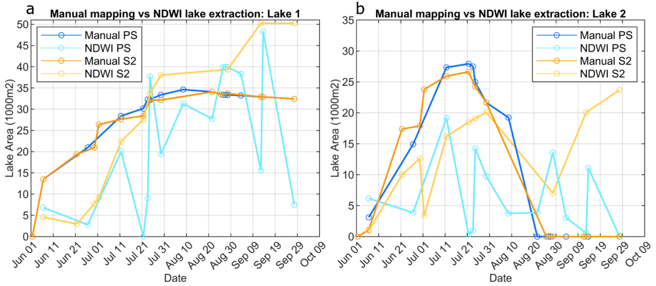
Fig. 6. Sub-seasonal development of the areas of Lake 1 (a) and Lake 2 (b) using manual vs. band-ratio (NDWI) mapping on the PlanetScope (PS) and Sentinel-2 (S2) images. Note the difference in the scales of the y-axis in the plots.
