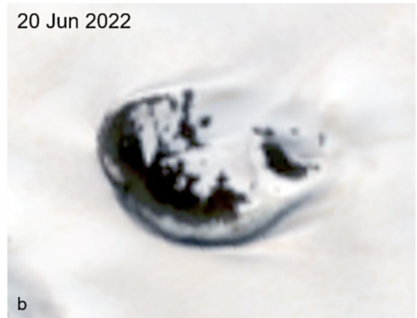
Fig. 11. Documentation of the drainage of Lake 4 between June 15 and June 20, 2022 (5 days). (a) shows the evidence of the filled Lake 4 on June 15, 2022, photographed during the fieldwork. Photo: Ursula Enzenhofer. (b) shows a PlanetScope satellite image from June 20, 2022, where the lake is empty.
