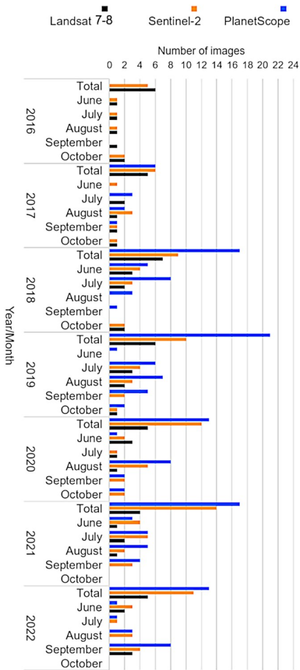
Fig. 3. Number of suitable images from Tystigbreen during the ablation season (June to October) for the period of 2016-22. All the images from October, except for the year 2017, are snow-covered and thus unfit for a reliable mapping.
