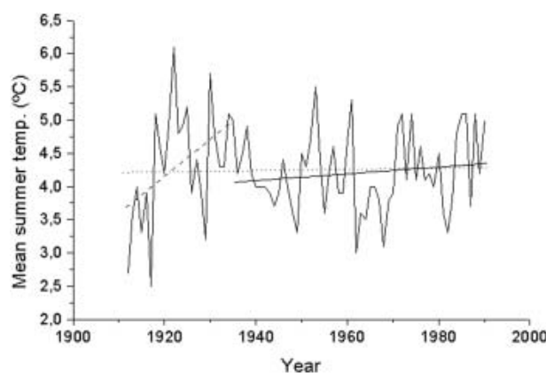
Fig. 5. Mean summer temperatures recorded at Isfjord Radio/Longyearbyen ( 78^{\circ}47' \text{ N} , 13^{\circ}38' \text{ E} ), 1912–90. The linear fits to the data for the full period (dotted line), the period 1936–90 considered in our volume-change estimates (solid line) and the period 1912–35 (dashed line) are plotted.
