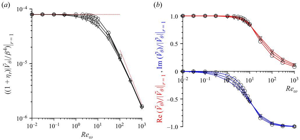
Figure 10. The measure (a) ((1 + \eta_r)|\tilde{V}_\theta|/\beta^4)|_{r=1} and (b) (\text{Re}(\tilde{V}_\theta)/|\tilde{V}_\theta|)|_{r=1} (red) and (\text{Im}(\tilde{V}_\theta)/|\tilde{V}_\theta|)|_{r=1} (blue) as a function of Re_\omega for viscosity ratio \eta_r \rightarrow 0 ( \circ ), \eta_r = 1.0 ( \triangle ), \eta_r \rightarrow \infty ( \nabla ). The definition of \tilde{V}_\theta is given in (2.16). The dotted red line on the left in (a) is the Re_\omega \ll 1 asymptotic result (4.6). The dotted red line on the right in (a) is the Re_\omega \gg 1 asymptotic result (4.7).
