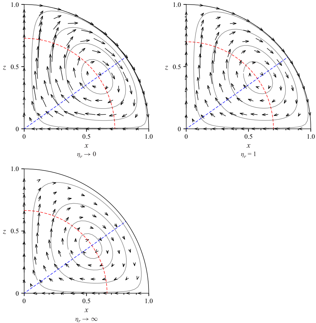
Figure 3. The velocity vectors (arrows) and the streamlines (dotted lines) for the flow in a drop due to an oscillating magnetic field for different values of the viscosity ratio \eta_r . The applied magnetic field is along the z axis, and x is along any direction in the equatorial plane. The solid quarter-circle is the boundary of the drop. The flow is radial ( \bar{v}_\theta = 0 ) along the dashed red quarter circle. The flow is in the azimuthal direction ( \bar{v}_r = 0 ) on the blue dashed line.
