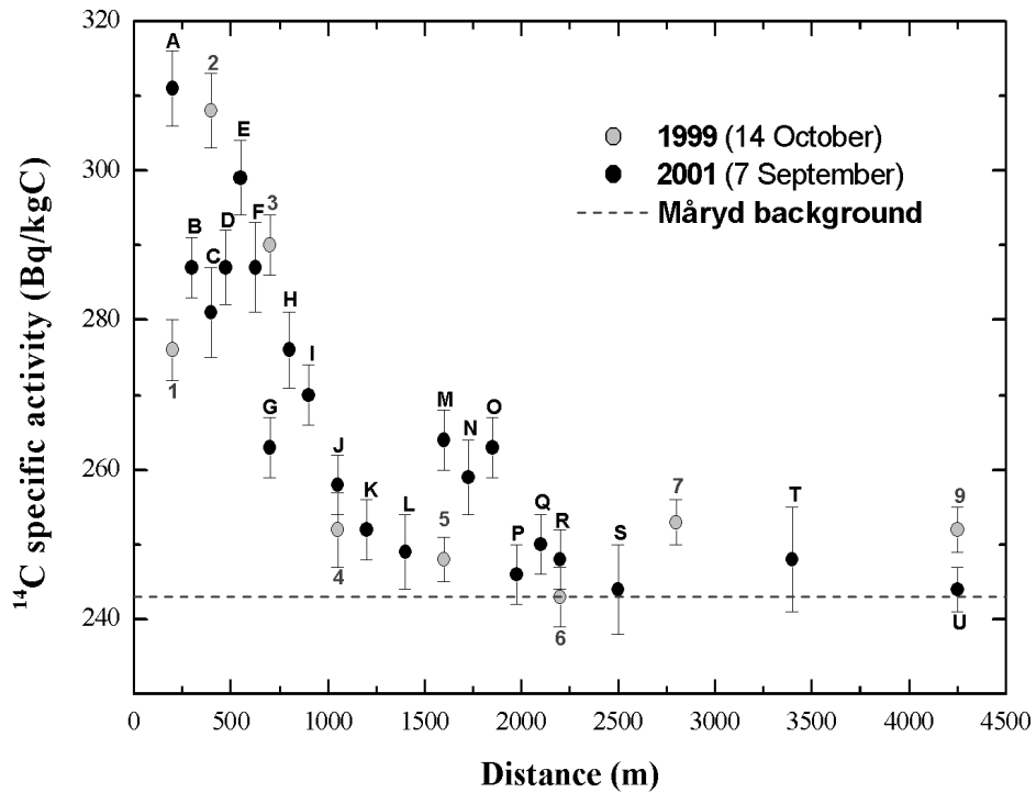
Figure 3 The 14 C specific activity (Bq/kg C) found in grass samples collected at various distances from the Cernavoda NPP. The background 14 C activity, 243 ± 2 Bq/kg C, measured in rush ( Juncus L. ) from Måryd, Sweden, is the mean value for the period 1999–2001. Figures and numbers refer to the sampling times and locations shown in Figure 1.
