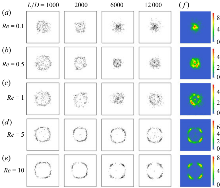
Figure 4. (a)–(e) Distributions of hydrogel particles ( d = 5.2 \mu\text{m} , D = 50 \mu\text{m} ) and (f) probability density functions (p.d.f.s) at L/D = 12\,000 ( L = 600 \text{ mm} ).
