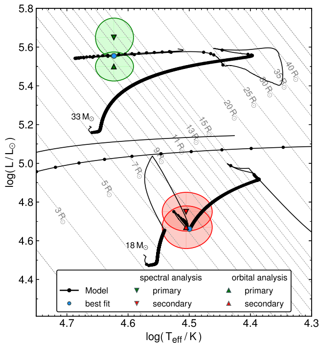
Figure 1. HRD showing the track of the binary evolutionary model (black line). The black dots on the tracks correspond to equidistant time-steps of 0.1 Myr to emphasize the most probable observable phases.
