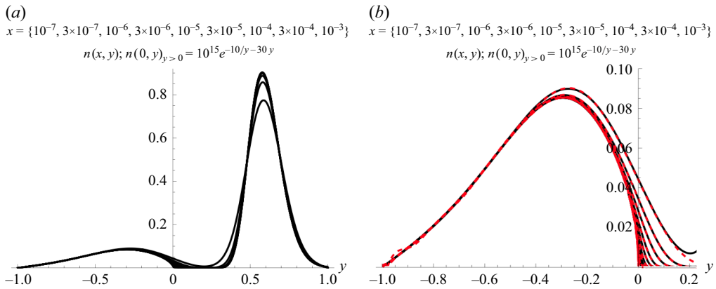
Figure 12. n(x, y) profiles obtained at several x values for initial condition n(0, y)_{y>0} = 10^{15}e^{-10/y-30y} , with L = 0.1 . Black lines are calculations with 500 modes. (a) full range. (b) Expanded view of the singular region. Dashed lines show n(x, y) = \sum t_k x^{1/6+k} h_{1/6+k}(y/x^{1/3}) , with t_k = \{0.18848, -1.4163, 8.9647, -44.732, 153.91, -347.18, 499.82, -440.42, 215.90, -45.033\} . Note the need for more modes near y = -1 for x = 10^{-3} .
