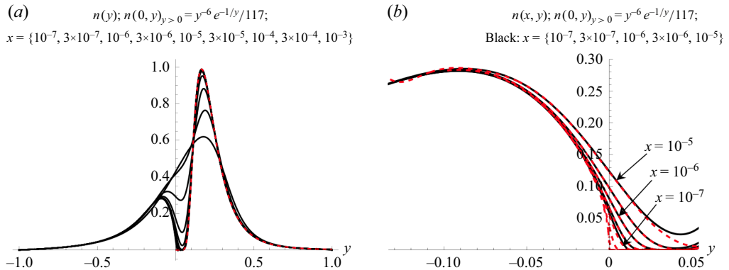
Figure 11. n(x, y) profiles obtained at several x values for initial condition n(0, y)_{y>0} = y^{-6}e^{-1/y}/117 , with L = 0.1 . Black lines are calculations with 500 modes. In (a) the dashed line is the initial condition. In (b) the dashed lines are n(x, y) = \sum t_k x^{1/6+k} h_{1/6+k}(y/x^{1/3}) , with t_k = \{1.16, -483, 4.28 \times 10^5, -3.482 \times 10^8, 1.613 \times 10^{11}, -3.16 \times 10^{13}, 1.04 \times 10^{15}\} .
