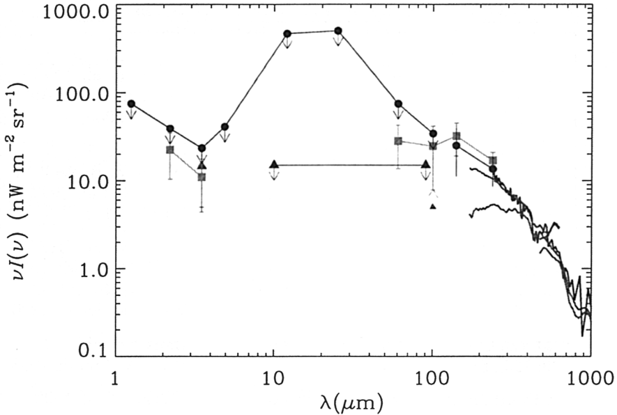
Figure 1. Summary of COBE-based CIB measurements. Detections are shown with 2\sigma uncertainties. Upper limits are given at the 2\sigma level. References are listed in Table 1. The curves at submillimeter wavelengths are from Fixsen et al. 1998 (dark wiggly curve from 200–1000 \mu\text{m} , representing the average of their three approaches); and Puget et al. 1996 (light curves from 150–1000 \mu\text{m} with break at \sim 500 \mu\text{m} : upper curve has no correction for emission correlated with ionized gas, lower curve has the correction).
