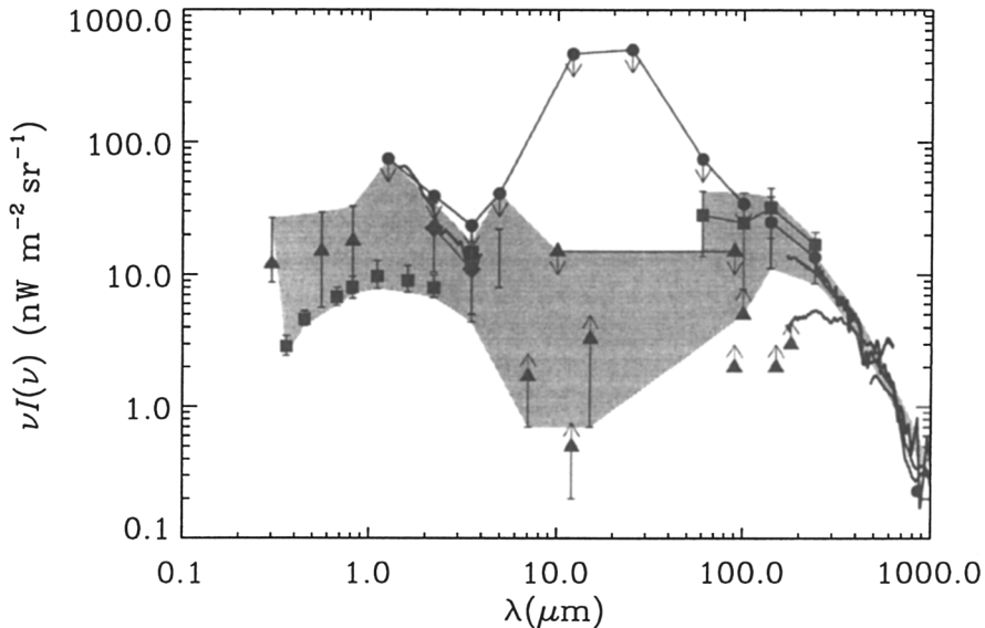
Figure 2. Measurements of the extragalactic background light. See text for references.
