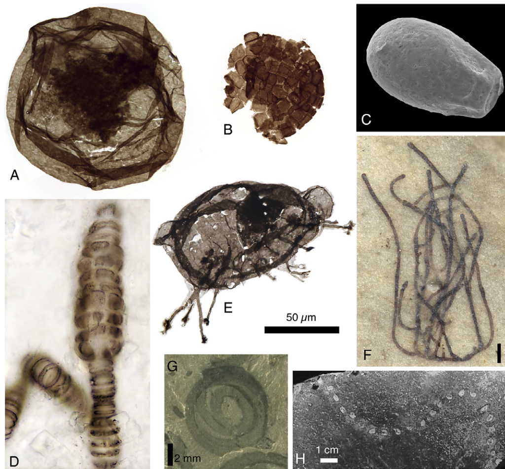
Figure 3. Examples of early eukaryote fossil species. A , Valeria lophostriata , Mesoproterozoic Battle Creek Fm, Bullita Group, Northern Territory, Australia. B , Satka favosa , Mesoproterozoic Wondan Hill Formation, Tjunna Group, Northern Territory, Australia. C , The vase-shaped microfossil Melanocyrtium hexodiadema , late Tonian Kwagunt Formation, Chuar Group, USA. D , Bangiomorpha pubescens , a red alga and the oldest widely accepted crown-group eukaryote, late Mesoproterozoic Hunting Formation, Canada. E , Tappania plana , early Mesoproterozoic Greyson Formation, Belt Supergroup, USA. F , Proterocladus antiquus , Nanfen Formation, late Mesoproterozoic/early Tonian Xihe Group, North China. G , Grypania spiralis , early Mesoproterozoic Greyson Formation, Belt Supergroup, USA. H , Horodyskia moniliformis , early Mesoproterozoic Appekuny Formation, Belt Supergroup, USA. Specimens in (A) and (B) from L.A.R.'s unpublished data, (C) from S.M.P.'s unpublished data. Specimen in (D) courtesy of N. Butterfield, from Butterfield (2000) Paleobiology 26:386–404, reproduced with permission from Cambridge University Press. E , Courtesy of N. Butterfield and Z. Adam, used with permission, Adam et al. (2017), Geology 45:387–390; permission conveyed through Copyright Clearance Center, Inc. F , Courtesy of Q. Tang, Tang et al. (2020), Nature Ecology and Evolution 4:543–549. G , Courtesy of M. Henderson, Henderson (2010) Master's thesis, University of Tennessee, Knoxville. H , From M. A. Fedonkin and E. L. Yochelson (2002), Smithsonian Contributions to Paleobiology 94; permission for use provided by Smithsonian Scholarly Press. Scale bars: (A–E) , 50 \mu m; (F) 100 \mu m; (G, H) as indicated.
