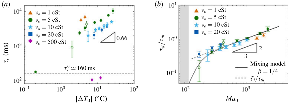
FIGURE 4. (a) Measurements of the residence time \tau_r as a function of the absolute value of the initial temperature difference |\Delta T_0| for the five different silicone oils considered. Open symbols represent the cases where \Delta T_0 < 0 . Each data point corresponds to an average over 30 drops and error bars are equivalent to two standard deviations. (b) The delay time \tau_d , non-dimensionalized by the characteristic thermal diffusion time \tau_{th} = R^2/\alpha_o , as a function of the initial Marangoni number Ma_0 . Symbols correspond to data from (a). The solid line is the theoretical prediction from the model described in § 3.2 with \beta = 1/4 . The dashed line is an approximate closed-form expression derived in the limit of t > \sqrt{3}/\dot{\gamma} .
