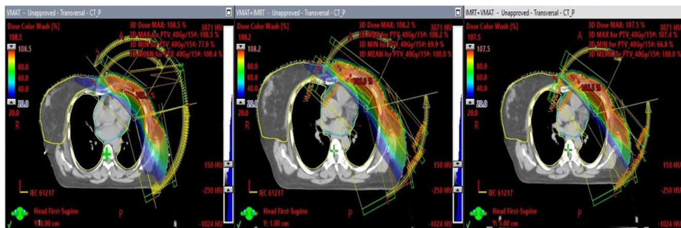
Figure 1. This illustration presents three transverse CT slices that depict the dose distribution of three distinct radiotherapy treatment plans: VMAT, VMAT+IMRT and IMRT+VMAT. The isodose lines extend from the highest dose percentage to a minimum of 20%.
