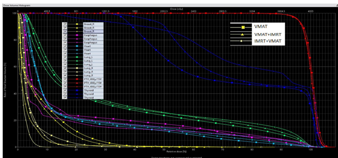
Figure 2. Illustrates a dose-volume histogram (DVH) comparing three different radiotherapy treatment techniques: VMAT, VMAT+IMRT and IMRT+VMAT.
