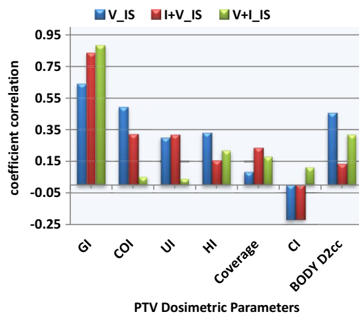
Figure 3. Correlation coefficients between individual and integrated scores in the PTV dosimetric parameters.
