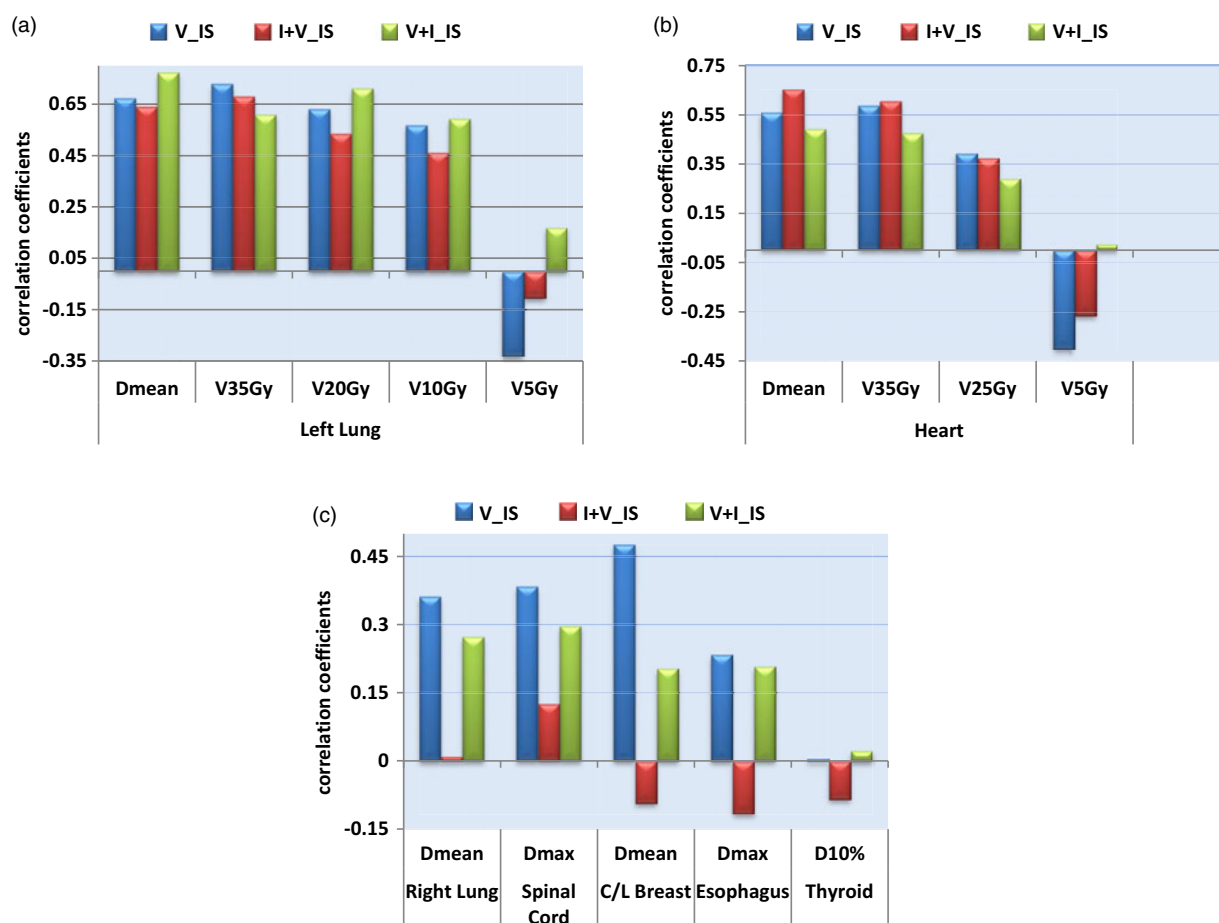
Figure 4. (a). Correlation coefficients between individual and integrated scores in the left lung. (b) Correlation coefficients between individual and integrated scores in the heart. (c) Correlation coefficients between individual and integrated scores in the OARs.
