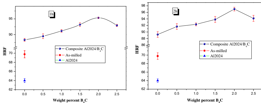
Figure 2. Hardness variation average values vs B 4 C weight percentage at different milling times: (a) 1 h and (b) 2 h.
