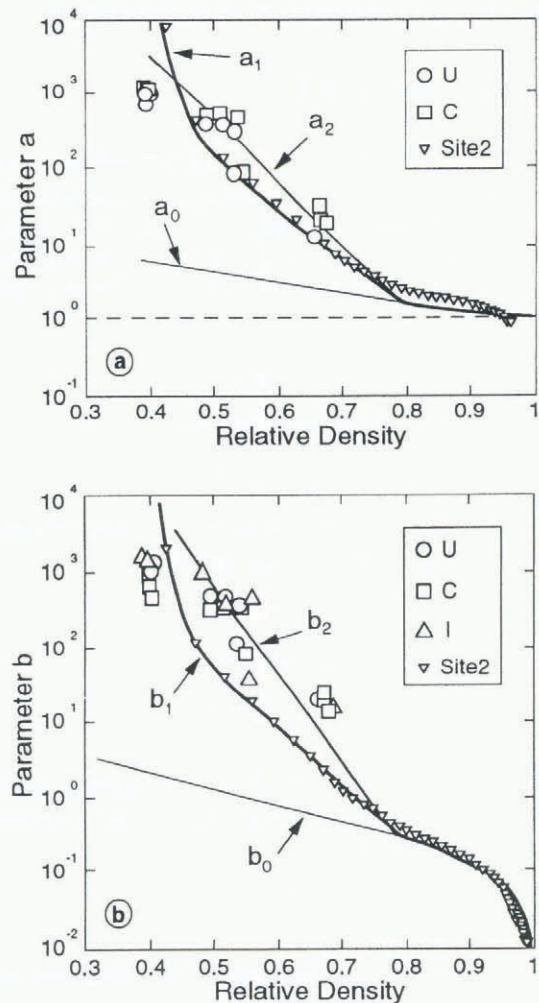
Fig. 2. Model parameters a (a) and b (b) vs relative density D . Solid lines show Duva and Crow's (1994) original functions ( a_0, b_0 ), and functions ( a_1, b_1 ), ( a_2, b_2 ) used in this study. Symbols show the values corresponding to Site 2 data and to Landauer's (1957) creep tests (U, uniaxial compression; C, confined compression; I, isotropic compression).
