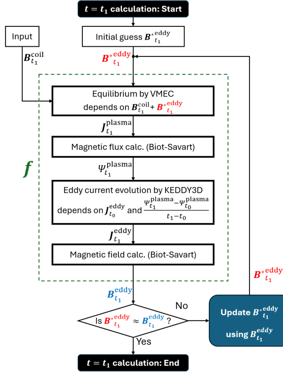
FIGURE 1. Flow of the evolution calculation to obtain the magnetic field produced by consistent eddy currents at t = t_1 . Here, J^{plasma} and J^{eddy} represent the plasma current and the eddy currents, B^{eddy} denotes the magnetic field produced by J^{eddy} , \psi^{plasma} denotes the magnetic flux produced by J^{plasma} and B^{coil} denotes the magnetic field produced by the coil current. The subscript of each variable indicates the value at the time step. The processes enclosed by the dashed line correspond to the calculations represented by function f in the text.
