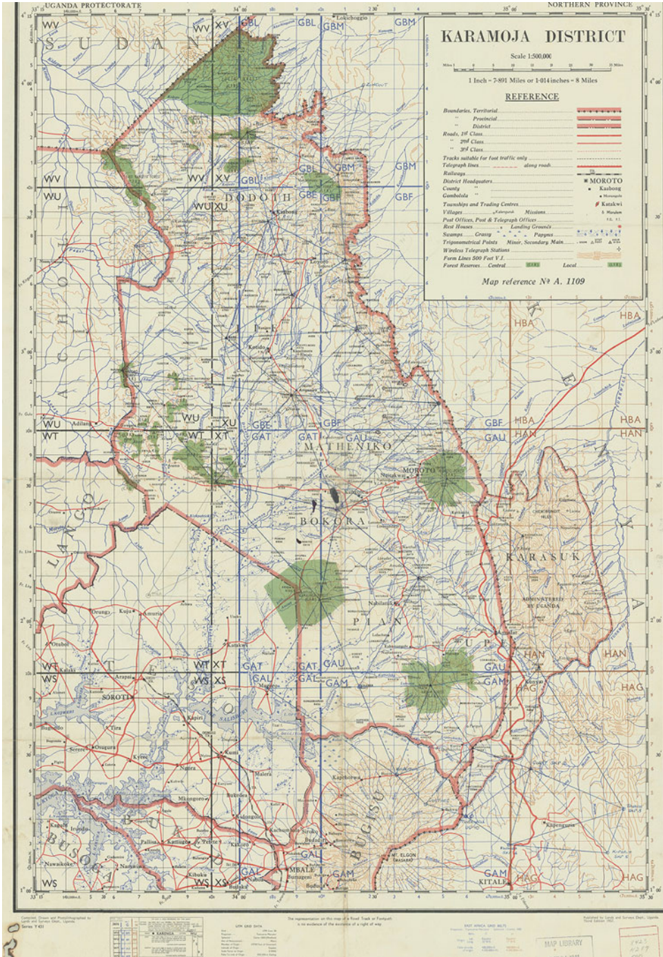
Figure 1. Karamoja District. Source: Uganda Department of Lands and Surveys. Map - Karamoja District, Uganda Protectorate, Northern Province . Kampala: Department of Lands and Surveys, 1957 (Courtesy of the Map and Data Library, University of Toronto).
