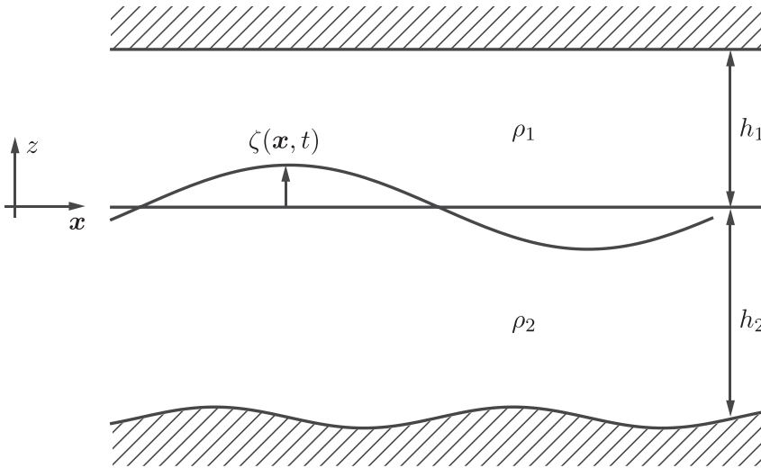
Figure 1. Internal gravity waves.
