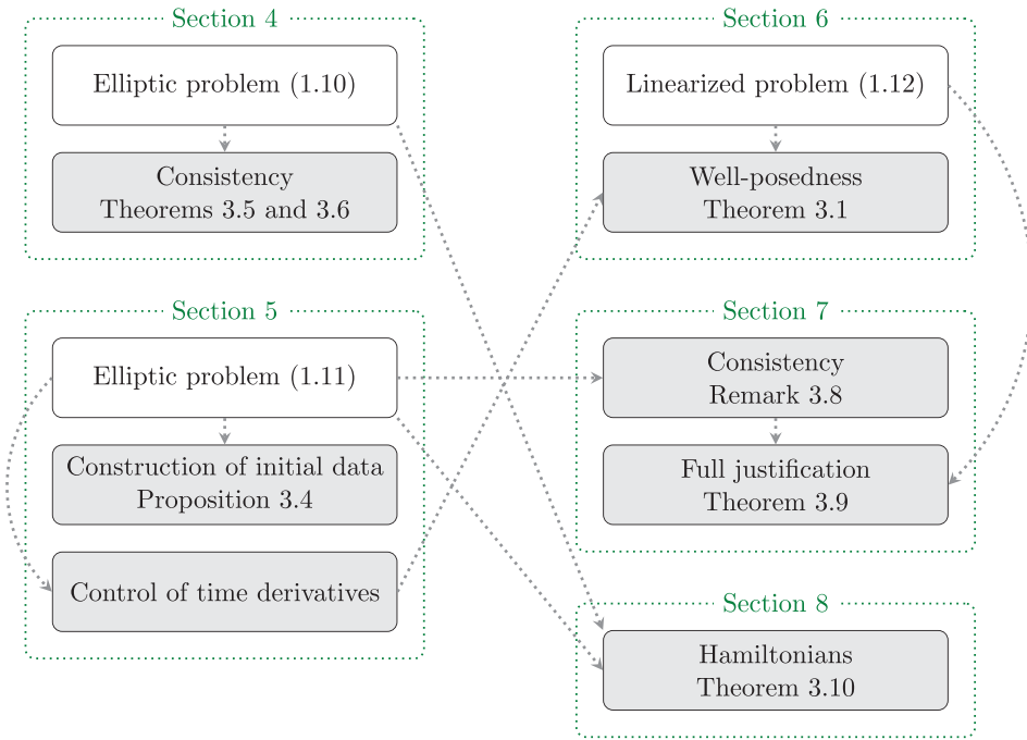
Figure 2. Articulation of the proofs.
