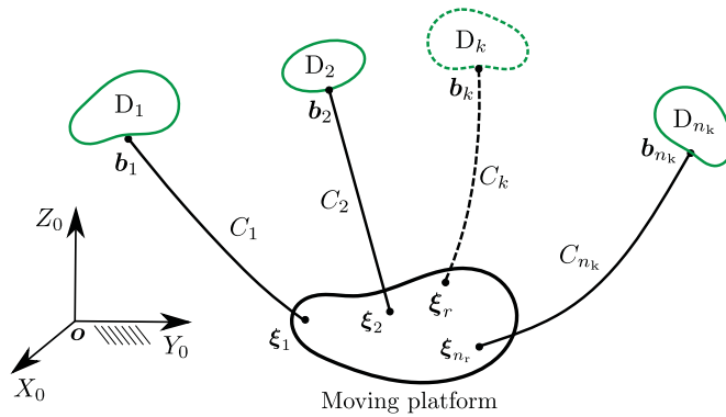
Figure 2. A schematic representation of a typical type II CDRP. The k th cable, labelled as C_k , is attached to the moving platform at \xi_r and connected to the driving mechanism D_k at \mathbf{b}_k . The point \mathbf{b}_k is known as the exit point (described in section 1).
