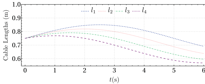
Figure 28. Variations in the input unstrained lengths of cables of the 4-4 CDRP, l_k, k = 1, \dots, 4 , associated with the feed rates given in Eq. (26).
