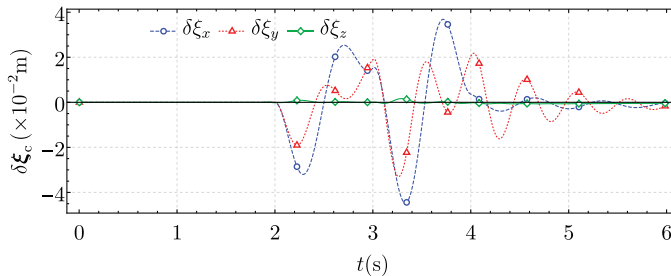
Figure 11. Variations in the error \delta\xi_c = \Delta\xi_c - \Delta b_k(t) with time. The scalar components of \delta\xi_c are denoted by \delta\xi_x , \delta\xi_y , and \delta\xi_z .
