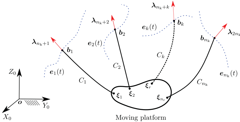
Figure 4. Representative trajectories e_k(t) of the exit points b_k of cables C_k in Type II CDRs. The reaction forces acting at the exit point b_k are denoted by \lambda_{n_k+k} .
