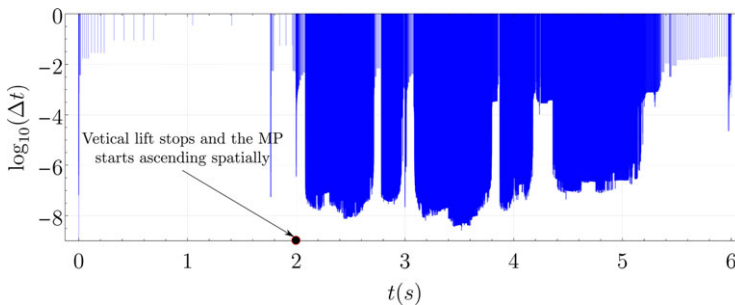
Figure 14. Variations in the step size \Delta t used by the solver ode15s at every instance of the simulation of the 4-4 CDRP for the input trajectories of the exit points of the cables b_i in Eq. (21). The sustenance of smaller steps can be seen during the spatial ascend and descend of the MP, that is, segments L_2 and L_3 in Fig. 7.
