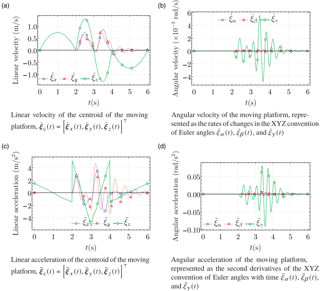
Figure 10. Variations in the linear, angular velocities \dot{q}_5(t) and accelerations \ddot{q}_5(t) of the moving platform of the 4-4 cable-driven parallel robot, corresponding to the inputs given in Eq. (21).
