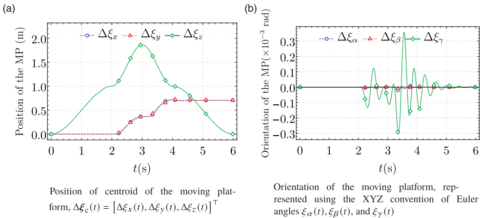
Figure 9. Variation in the configuration of the moving platform of the 4-4 cable-driven parallel robot, \Delta q_5(t) = q_5(t) - q_5(0) , for the inputs given in Eq. (21).
