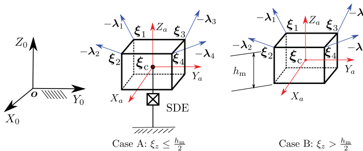
Figure 35. Changes in the model of the cuboid MP of 4-4 CDRP based on its state of contact with the ground. Case A is used when it is in contact with the ground and case B when it is not in contact. The symbol \xi_z represents the vertical position of the centre of mass of the MP with respect to the frame \mathbf{o}-X_0Y_0Z_0 .
