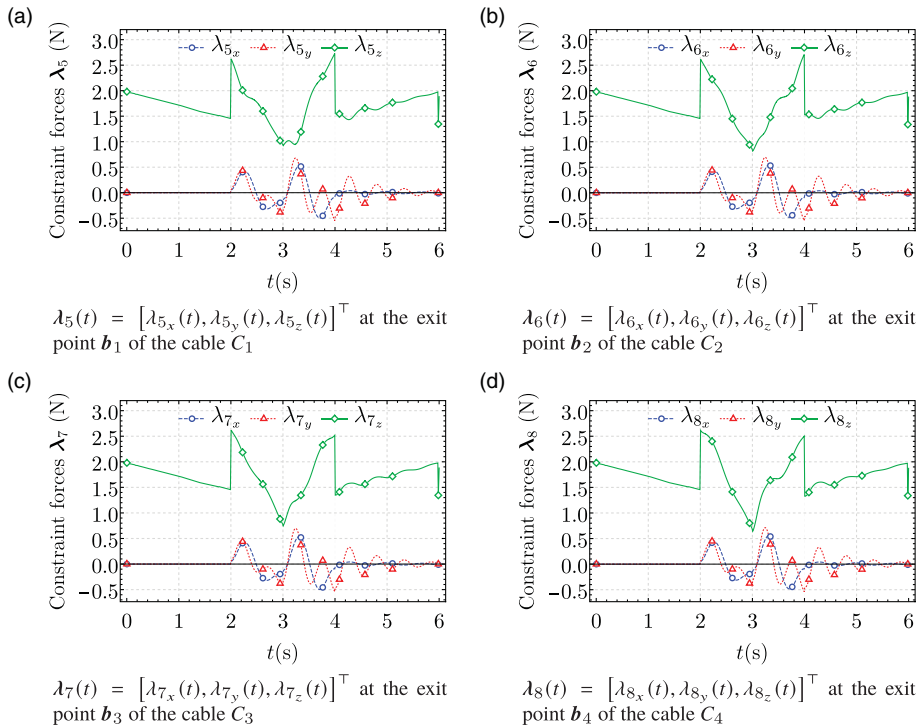
Figure 13. Variations in the values of components of the reaction forces \lambda_i, i = 5, \dots, 8 , with time, corresponding to the simulation of the 4-4 cable-driven parallel robot for the inputs given in Eq. (21).
