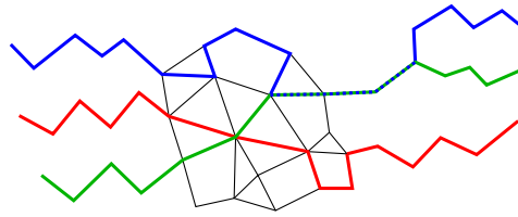
FIGURE 1 (colour online). A vertex space of Z . The thickened lines represent attaching maps of non-compact edge spaces, each of which being homeomorphic to \mathbb{R} .
