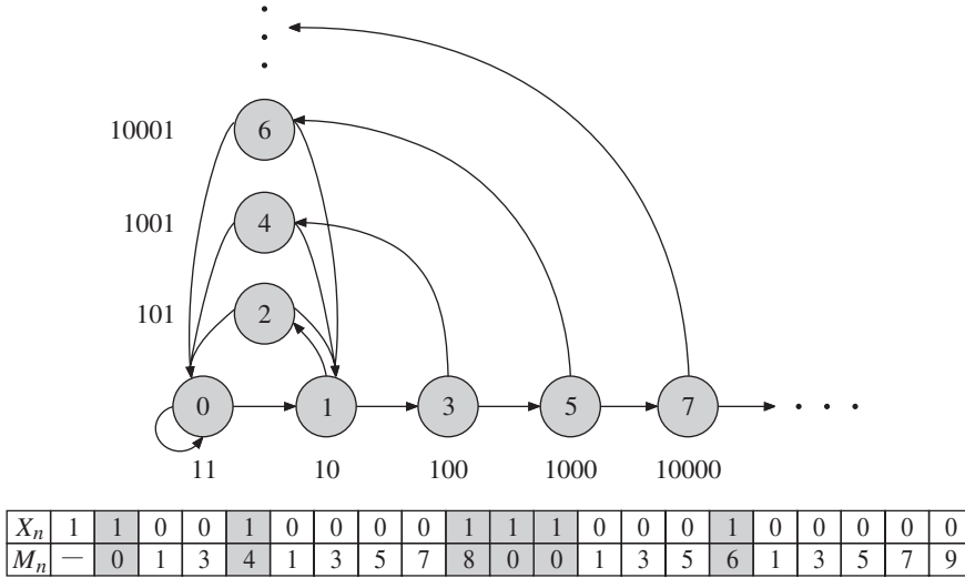
FIGURE 1: Construction of the Markov chain (M_n) , with an example sequence showing the correspondence with X_n .
