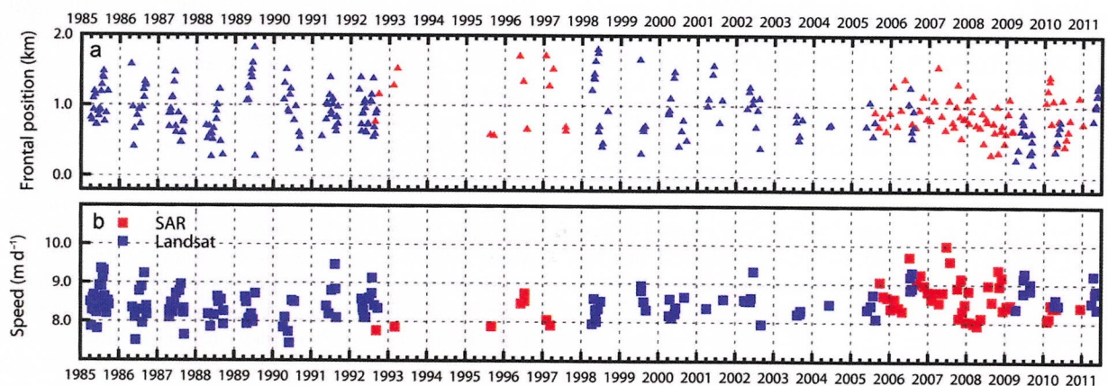
Fig. 3. (a) Centre front position relative to most retreated position based on Landsat images and ERS-1 and -2 SAR and Envisat ASAR image mode scenes. (b) Complete time series of velocity magnitudes extracted from a point 5 km upstream of the glacier front (see flag in Fig. 2). In both (a) and (b) Landsat measurements are in blue and SAR measurements are in red.
