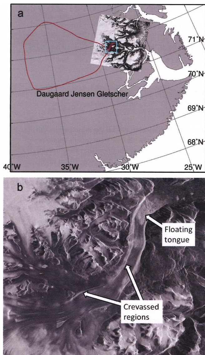
Fig. 1. (a) Location of Dugaard Jensen Gletscher. The image overlain is a Landsat image. The cyan box shows the region covered in Figure 2 and the red outline shows the catchment boundary. (b) Subsection of an ERS-1 SAR image acquired on 17 March 1993. The image covers approximately 60\text{ km} \times 60\text{ km} and is in slant-range and azimuth coordinates. Heavily crevassed regions, such as the floating tongue and marginal shear regions, enhance the backscatter and are visible as bright regions.
