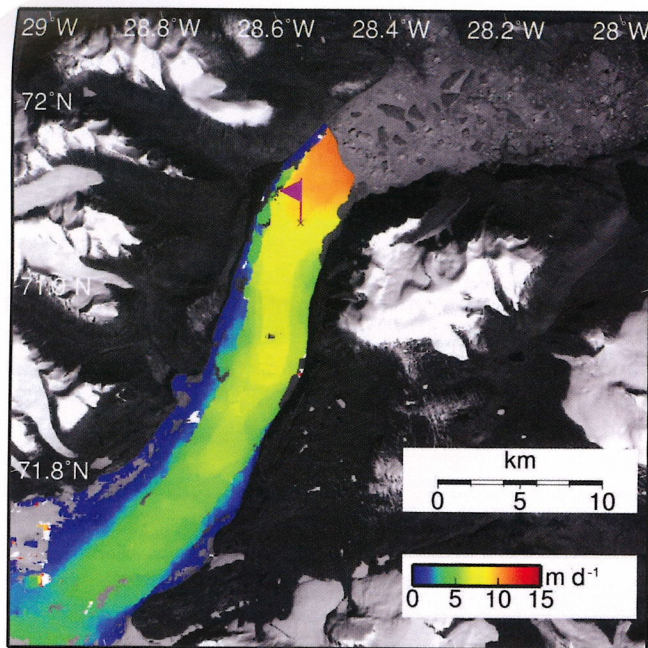
Fig. 2. Results of feature tracking between Landsat-5 images acquired on 18 July and 19 August 1986. The flag marks the location of the extraction point for the time series of velocities presented in Figures 3 and 4.
