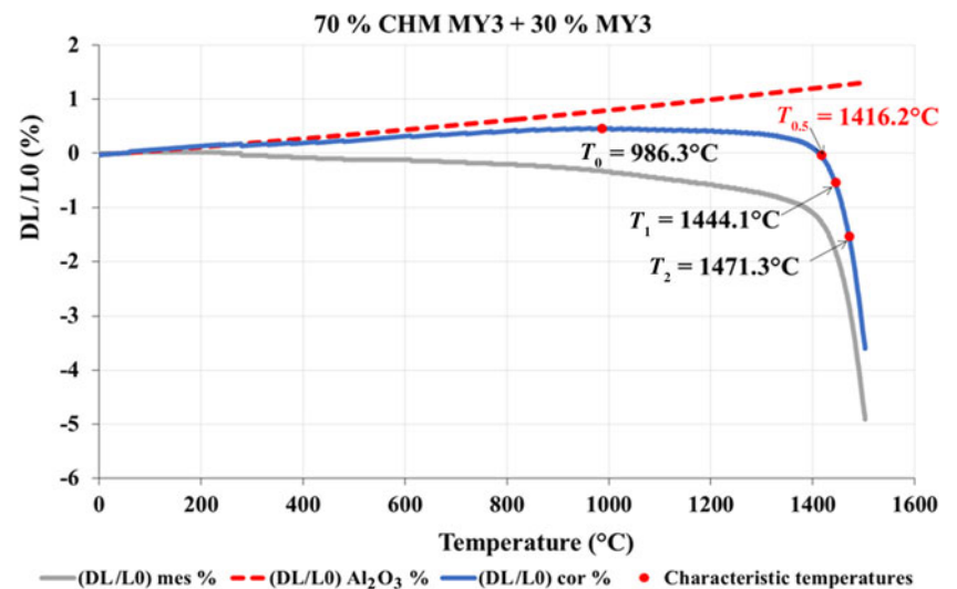
Figure 9. Example of a refractoriness under load curve for MY3. DL/L0 = the rate of material expansion/shrinkage; DL/L0 cor % = the corrected rate of material expansion/shrinkage; DL/L0 mes % = the measured rate of material expansion/shrinkage.
