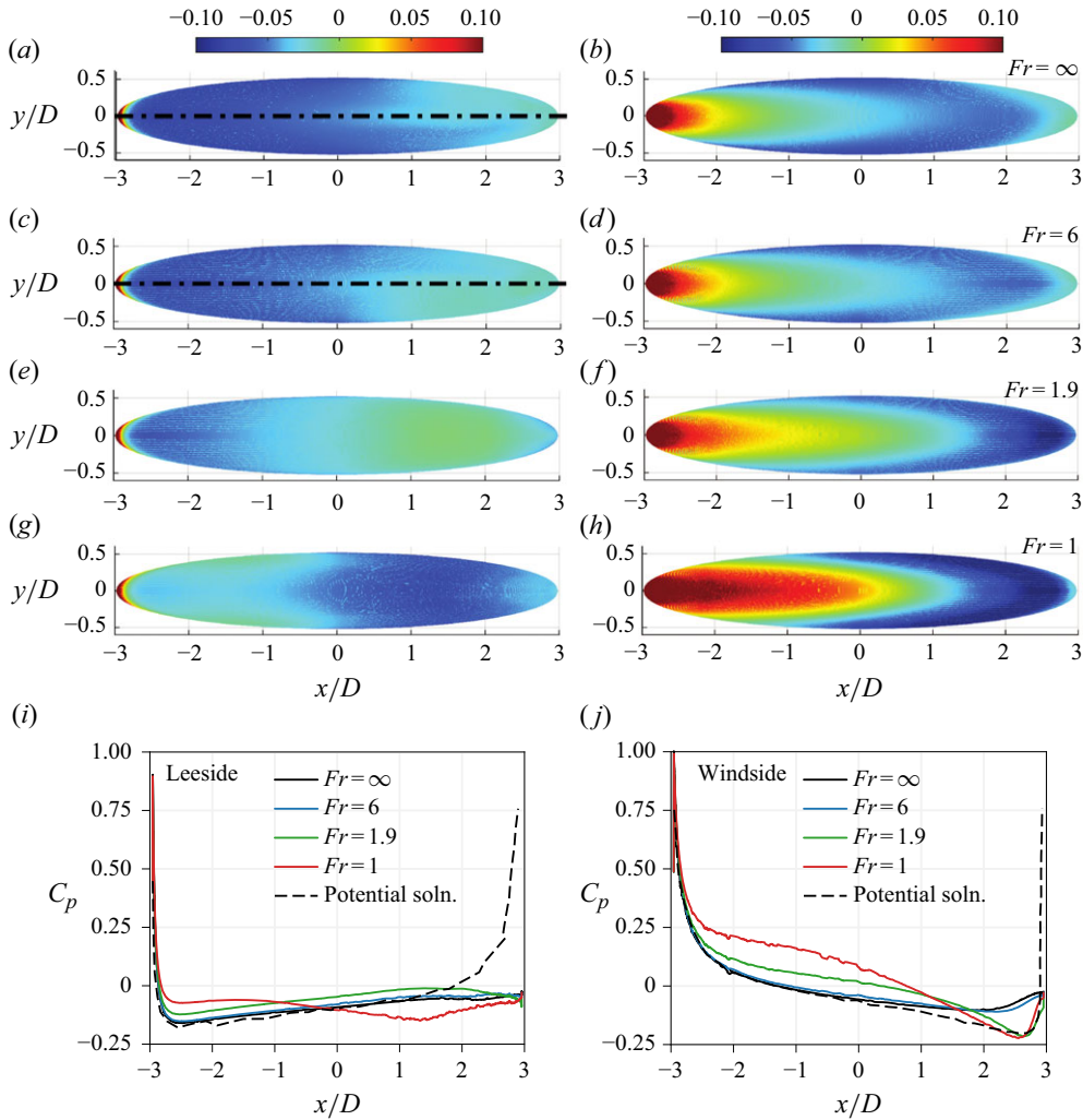
Figure 8. Pressure contours on the (a,c,e,g) leeward and (b,d,f,h) windward side of the spheroid. Dashed line in panels (a) and (c) corresponds to y/D = 0 . Variation of C_p(x) on the (i) leeward and (j) windward side of the body surface in the y/D = 0 plane. The potential flow solution for C_p(x) , obtained from Piquet & Queutey (1992), is also shown as a dashed line in panels (i) and (j).
