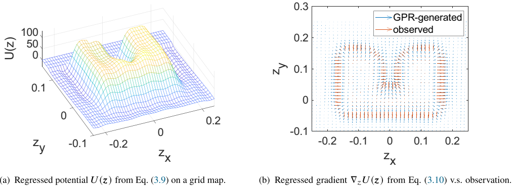
Figure 6. Regressed potential U(\mathbf{z}) and gradient \nabla_{\mathbf{z}} U(\mathbf{z}) .
