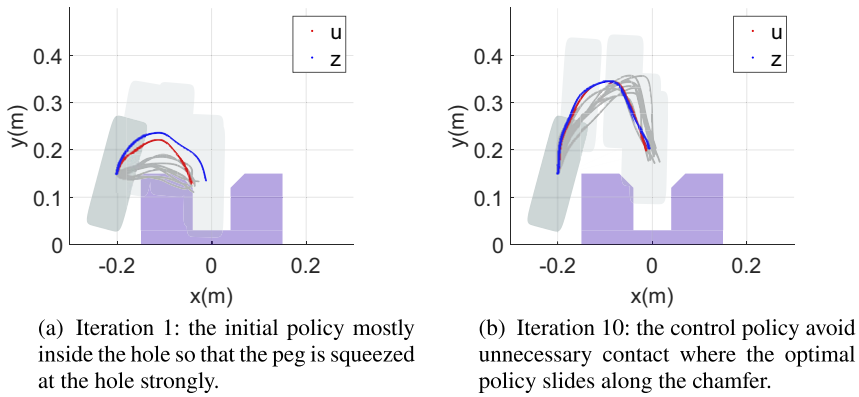
Figure 10. Iterations during BBO: the red curve denotes the optimal control policy u(t) in this iteration, the blue one denotes z(t) , and the gray curves represent the nonoptimal explorations in each iteration of BBO.
