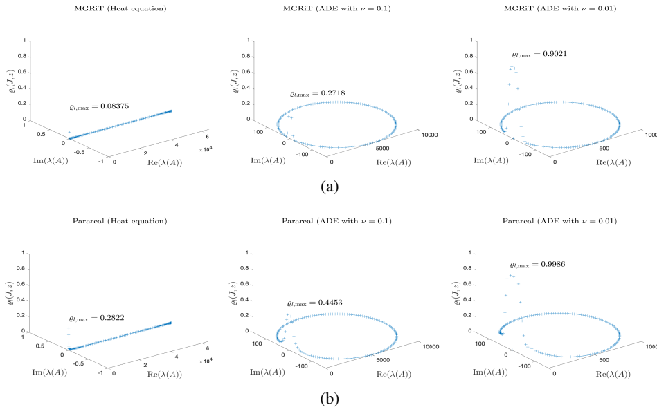
Figure 4.9. The distribution of \varrho_l(J, z) for z \in \sigma(\Delta T A) for the heat equation and the advection–diffusion equation (ADE) with two values of the diffusion parameter \nu . (a) MGRiT, (b) Parareal. In each panel, \varrho_{l, \max} = \max_{z \in \sigma(\Delta T A)} \varrho_l(z) .
