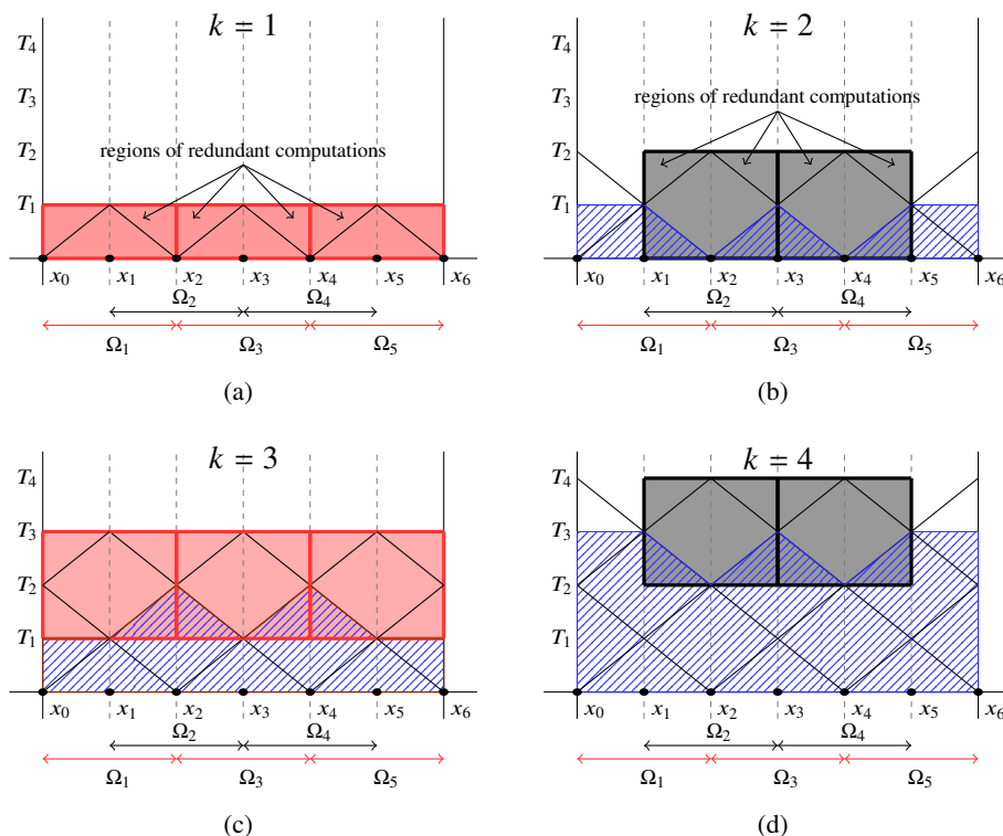
Figure 3.2. Illustration of red–black SWR with generous overlap.
