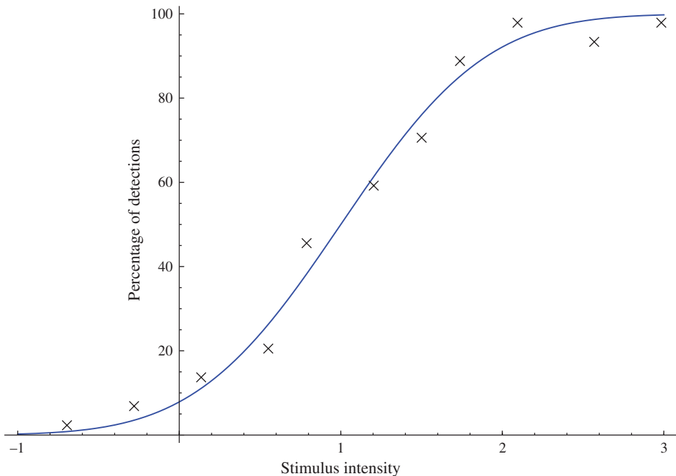
Figure 2.21 The most basic psychometric function . For this example, as the stimulus intensity is increased, the percentage of people detecting the phenomenon increases. The point along the curve that corresponds to 50 percent indicates a critical threshold or boundary in the stimulus intensity. The curve here corresponds to the cumulative distribution function of the error model (often assumed to be Gaussian).
