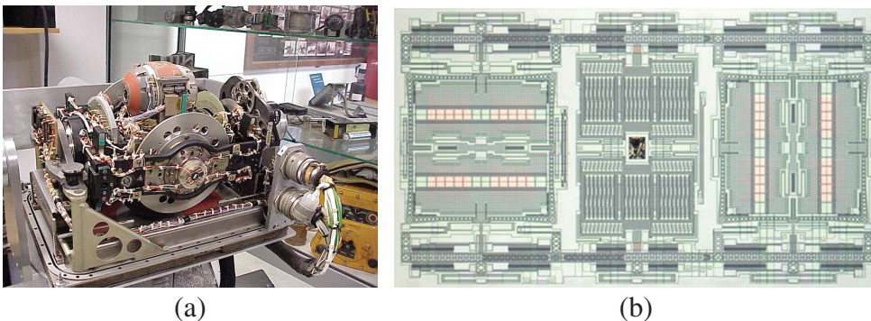
Figure 2.9 Inertial measurement units (IMUs) have gone from large, heavy mechanical systems to cheap, microscopic MEMS circuits. (a) The LN-3 Inertial Navigation System, developed in the 1960s by Litton Industries. (b) The internal structures of a MEMS gyroscope, for which the total width is less than 1 mm.
