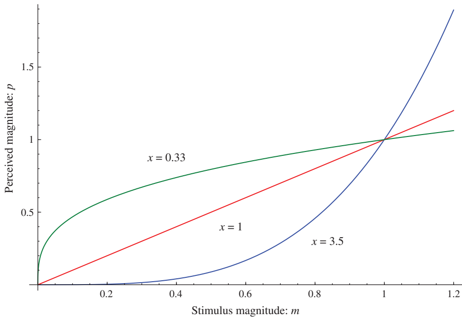
Figure 2.22 Steven's power law (2.1) captures the relationship between the magnitude of a stimulus and its perceived magnitude. The model is an exponential curve, and the exponent depends on the stimulus type.
