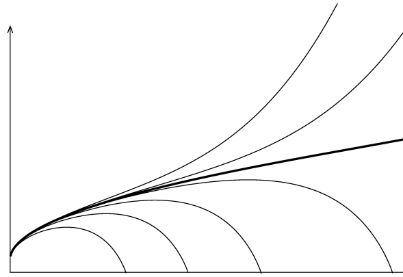
Figure 1: The structure of the solutions to (2.1) for p = 3/2 and q = 7/4 . When h(0) is small, the maximal domain of the solution is bounded. On the other hand, if h(0) is large, then the solution is convex for sufficiently large arguments. The bold curve corresponds to the graph of the solution described in Theorem 2.1.
