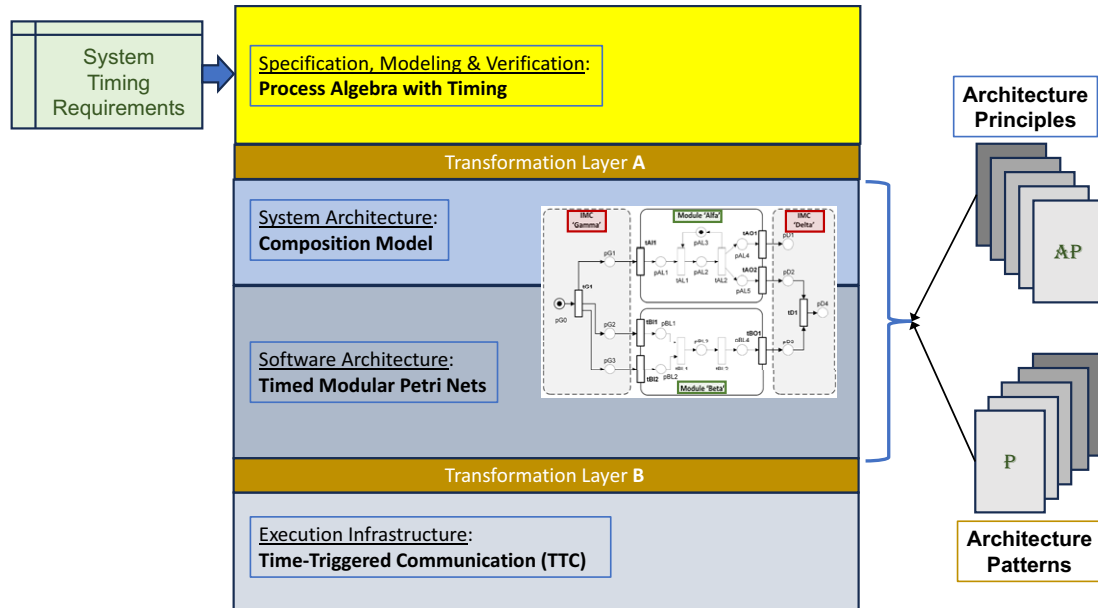
Figure 6. Software architecture.
