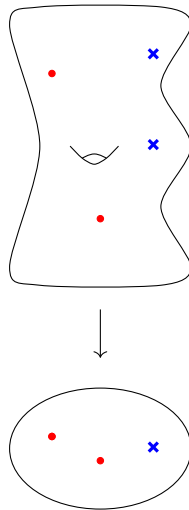
Fig. 1. A curve C \rightarrow \mathbb{P}^1 in \overline{\mathcal{H}}_{1,d,4,2} with n = 4 markings in C of which r = 2 lie in the fibre over the same point of \mathbb{P}^1 .
