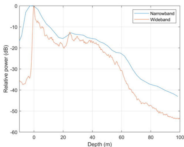
Fig. 4. Along-track average return power of the echograms in Figure 3. The first density band reaches a depth of \sim 20 m, the second density band extends from \sim 20 to \sim 50 m, and final density band extends below 50 m.
