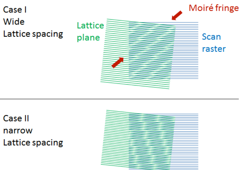
Figure 1. Schematic illustration of scanning moiré fringe method used in this study (rotation moiré). Scan raster (blue) is slightly tilted from lattice plane (green). When lattice spacing is changed (case 1 and case 2), the angle and spacing of moiré fringes (as shown by red arrows) are changed largely.
