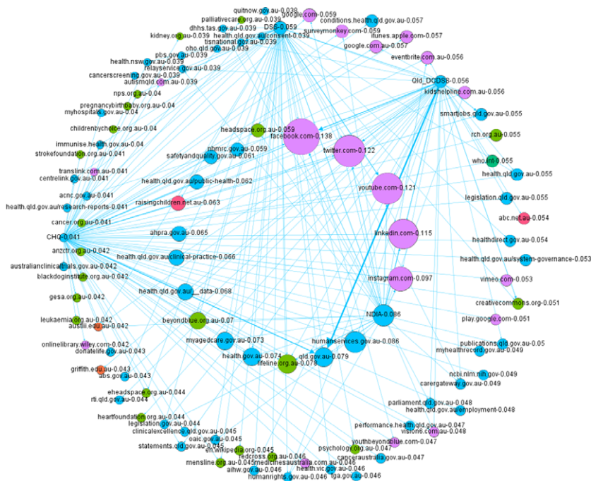
Figure 2. Top 100 authority scores from the full NDIA network
