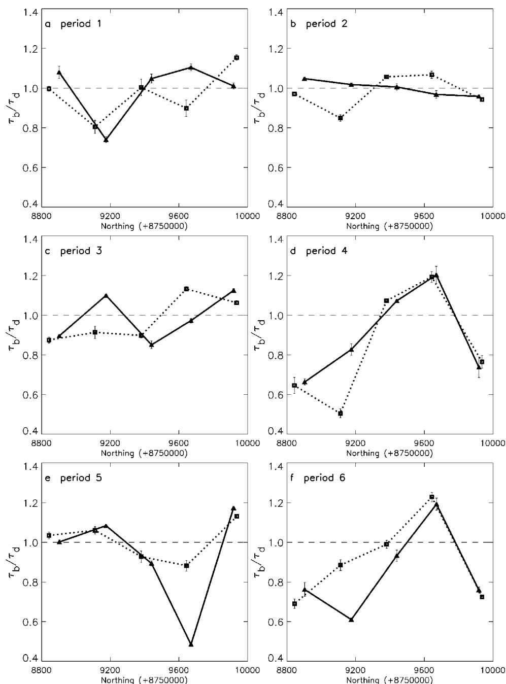
Fig. 5. Ratio of basal drag to driving stress ( \tau_b/\tau_d ) in the tongue. The glacier terminus is to the right (increasing northing). Solid lines and triangles represent the western line of force-balance blocks, while dotted lines and squares represent the eastern line of blocks. Where \tau_b/\tau_d < 1 , some resistance to flow comes from non-local sources (a slippery spot). Where \tau_b/\tau_d > 1 , flow is driven by forces in addition to the driving force (a sticky spot). Error bars representing the standard deviation are shown. (a) Period 1 (5–9 July); (b) period 2 (9–15 July); (c) period 3 (15–20 July); (d) period 4 (20–23 July); (e) period 5 (23 July–6 August); and (f) period 6 (6–9 August).
