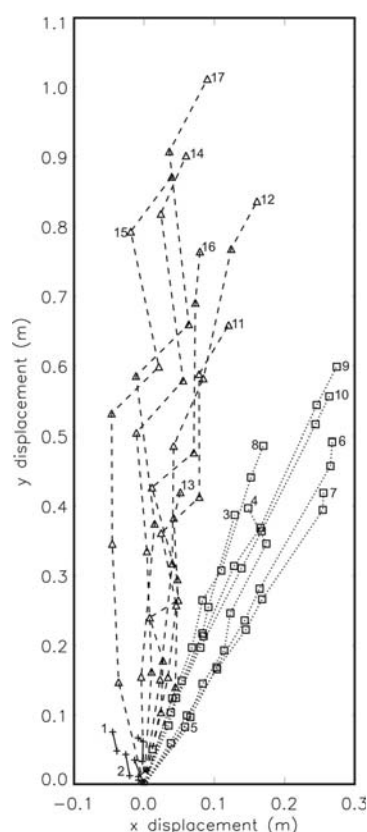
Fig. 2. Displacement of velocity stakes throughout the summer 1999 season for all stakes (numbered). Crosses and solid lines indicate northwest-trending stakes in the lower tongue (1 and 2); squares and dotted lines indicate northeast-trending stakes in the middle tongue (3–10); triangles and dashed lines indicate northerly-trending stakes in the upper tongue (11–17).
