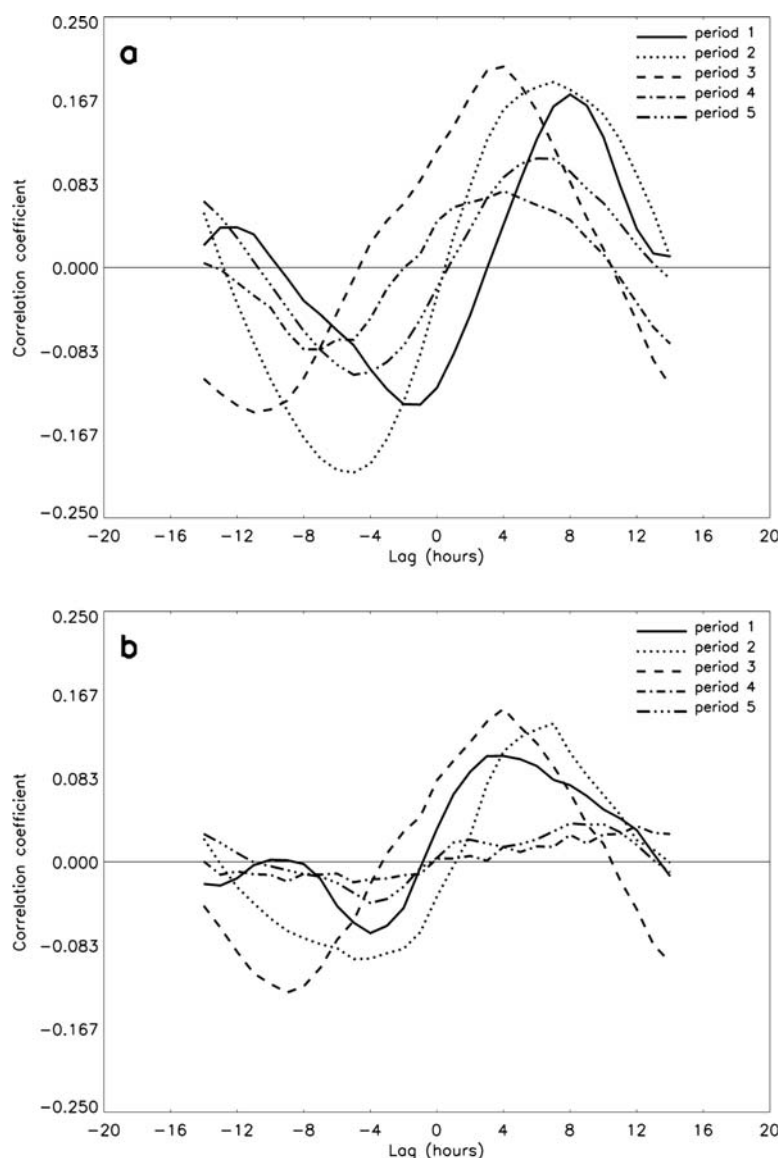
Fig. 9. The correlation coefficients between air temperature and discharge associated with different lag times in the western outlet (a) and eastern outlet (b), in periods 1–5, when a full discharge record was available. Data were differenced to remove trends, and smoothed over a 5 hour period, using a centred 5 hour moving average. For each period, the greatest correlation coefficient indicates the average time lag between melting at the surface and discharge in the proglacial streams.
