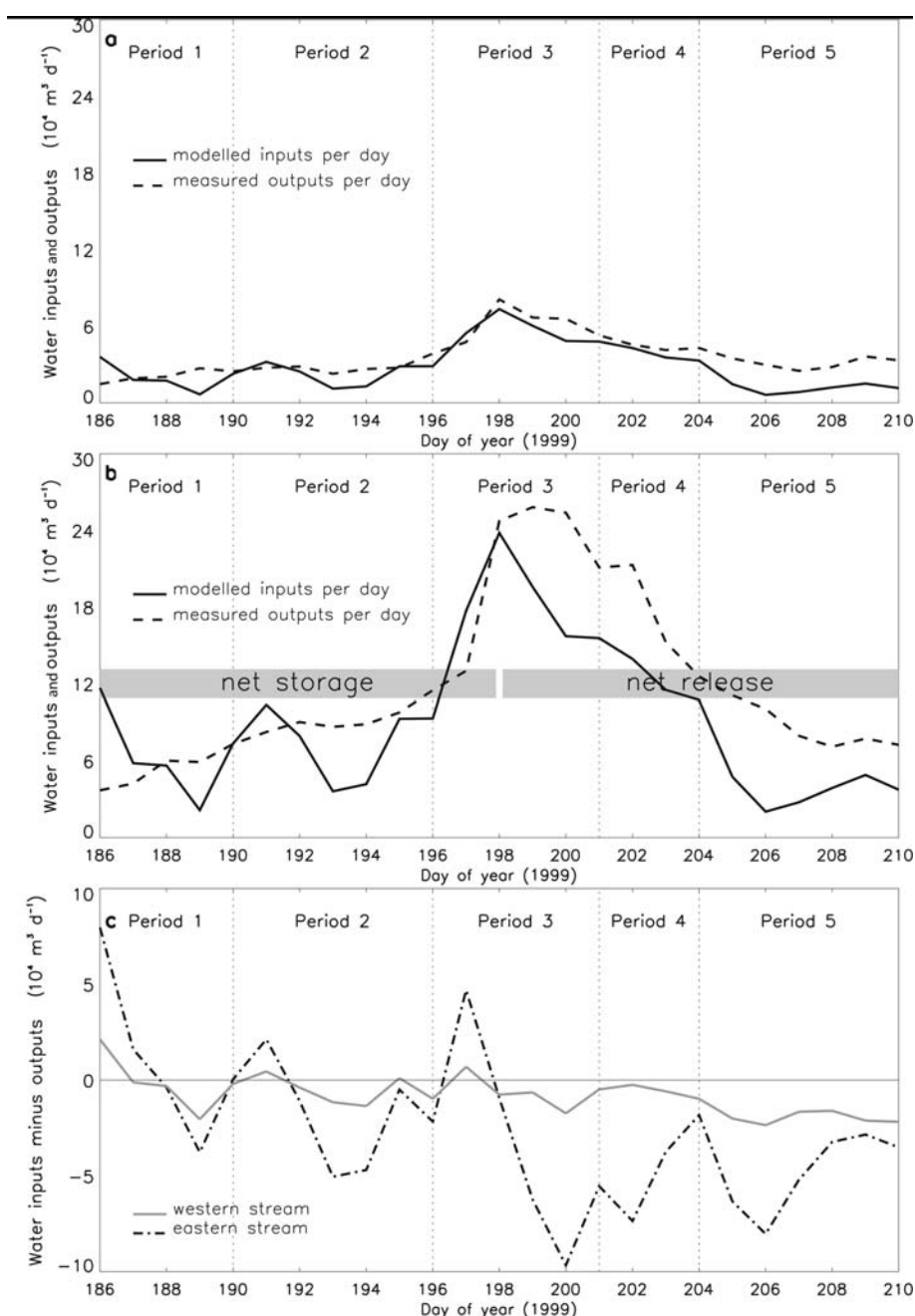
Fig. 8. (a, b) Modelled and measured daily water inputs to and outputs from the western stream (a) and eastern stream (b). (c) The difference between inputs and outputs in the eastern and western streams. A positive difference indicates less water exiting the glacier than would be expected given the recorded temperatures, and thus water going into storage; while a negative difference indicates more water exiting the glacier than would be expected, and thus water being released from storage. Water balance is shown up to day 210 only, since there was no eastern discharge record after this.
