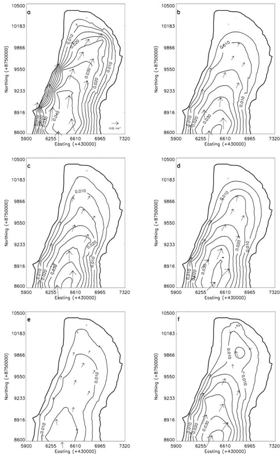
Fig. 3. Horizontal xy surface velocities (m d -1 ) in the tongue. Arrows indicate xy velocity azimuth, and their size is proportional to the measured xy velocity magnitude (size guide shown in (a)). A linear kriging interpolation scheme was used to derive velocity contours. Contours are marked every 0.005 m d -1 and labelled every 0.01 m d -1 . At the ice margin, xy velocities are set to zero. (a) Period 1 (5–9 July); (b) period 2 (9–15 July); (c) period 3 (15–20 July); (d) period 4 (20–23 July); (e) period 5 (23 July–6 August); and (f) period 6 (6–9 August).
