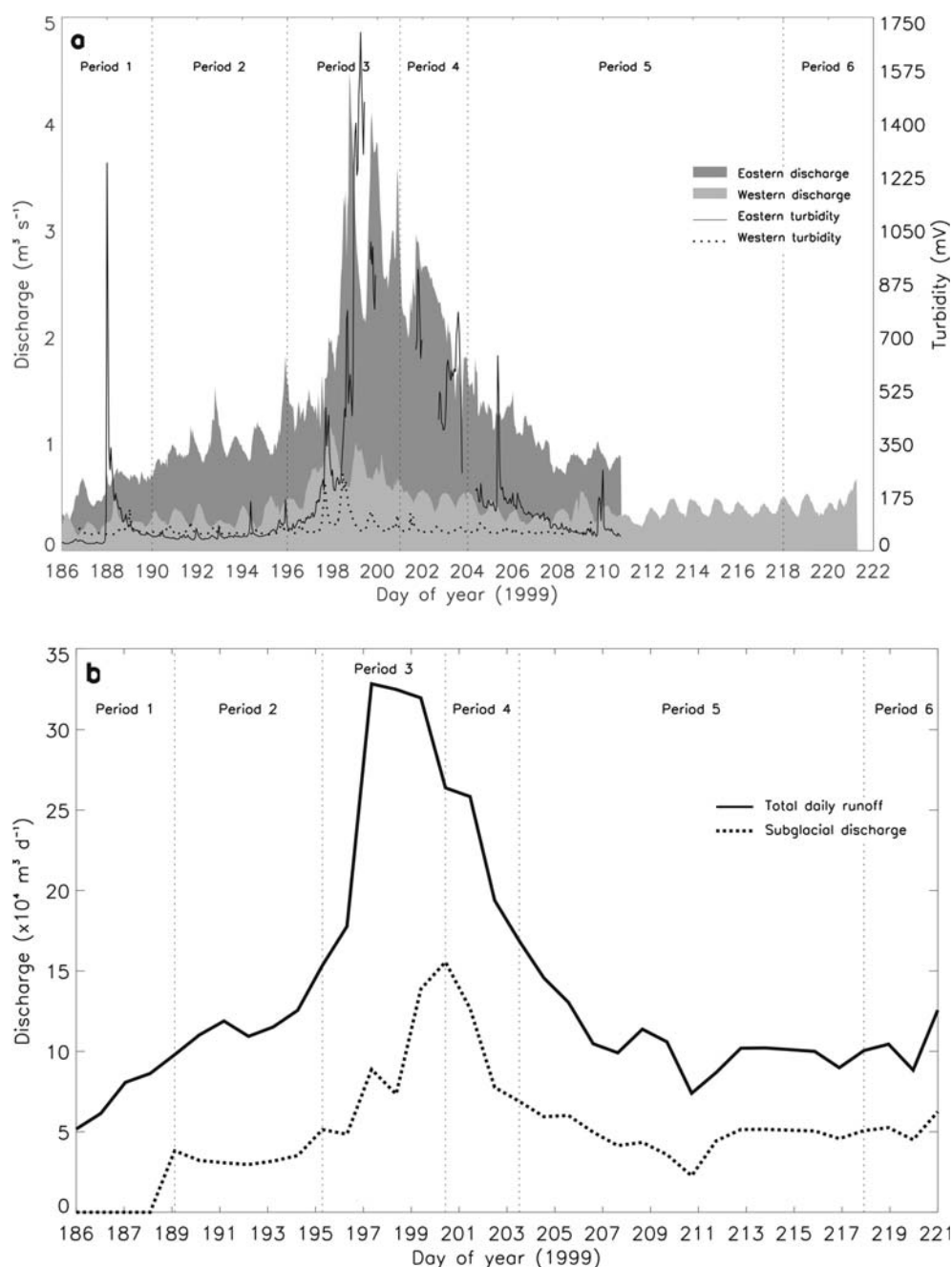
Fig. 7. (a) Proglacial discharge (in \text{m}^3 \text{s}^{-1} ) and turbidity (in mV, logged directly from the turbidity sensor) time series in 1999 for the eastern and western outlets. The six intra-summer periods are marked. (b) Total (measured) daily runoff and (modelled) subglacial discharge (both in \text{m}^3 \text{d}^{-1} ).
