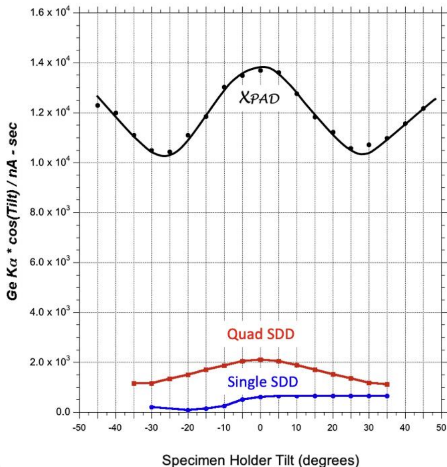
Figure 2. Experimental Penumbra effects as a function of specimen holder tilt for Argonne Instruments: Single 60 mm 2 SDD, Quad 30 mm 2 SDD and XPAD
