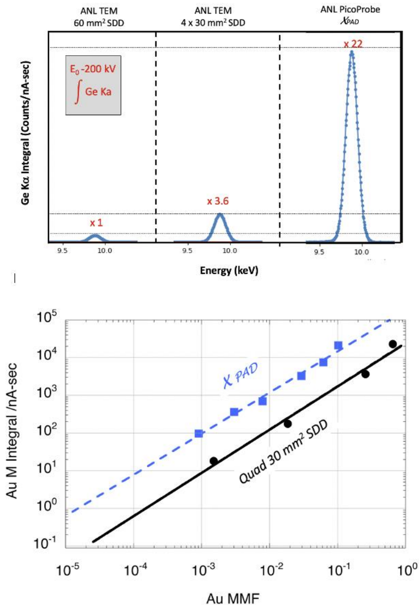
Figure 1. (a) Normalized performance of XEDS Collection for Ge K \alpha (Integrated Counts/nA-sec) from a 20nm thick ultra-nanocrystalline Ge film on SiN x for Single, Quad and XPAD systems. (b) Improvement of MMF of Au nanoparticles on SiN x at 80 kV. Solid line Quad 30 mm 2 SDD, Dashed line XPAD.
